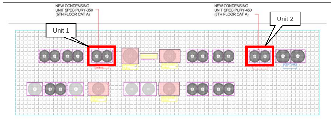
Proposed Plant Arrangement Roof Level, (c/o Air Conditioning Design Ltd).
