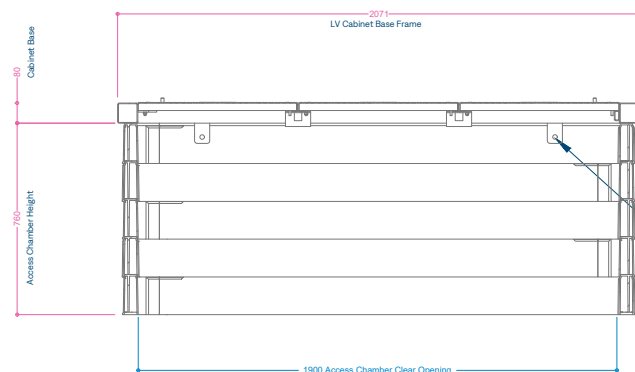
NAL Cabinet Base System – Schneider LV Pillar Cabinet Base
