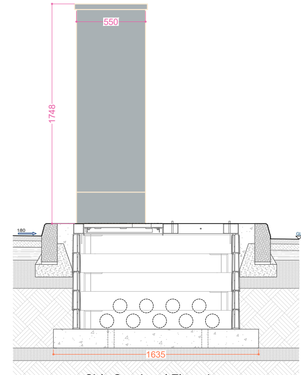
Side Sectional Elevation
