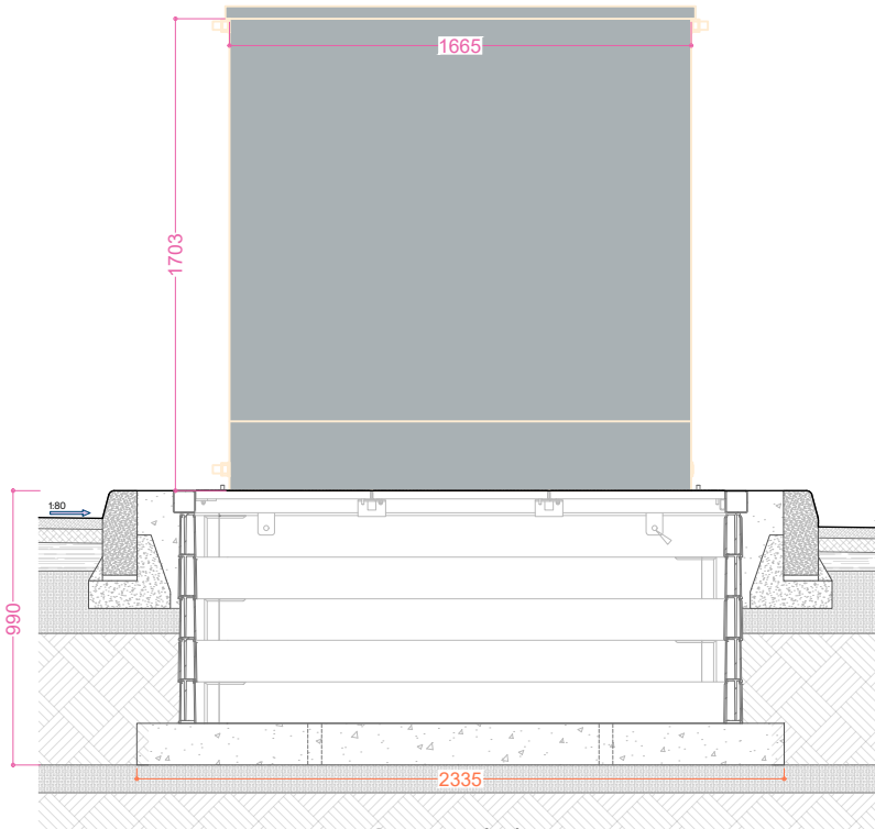
Rear Sectional Elevation
