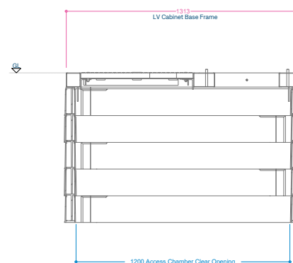
Rear Sectional Elevation
