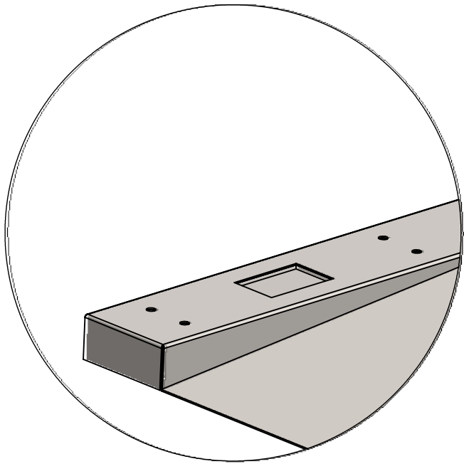
DETAIL A LIFELINE UNIT SHOULD ALIGN WITH END OF BASE PLINTH ASSEMBLY SCALE 1 : 5
