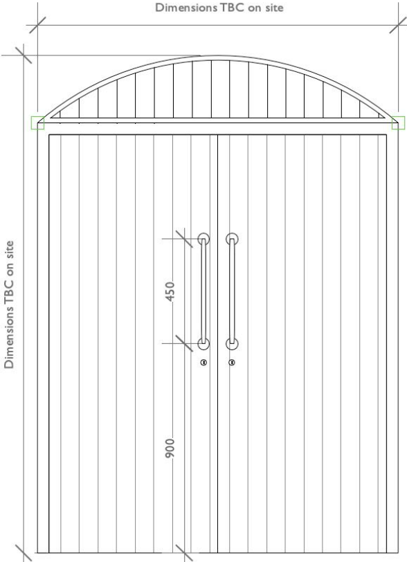
Proposed - Fire door and surround (refer to drawings T(710) and T(400,401) for further details
