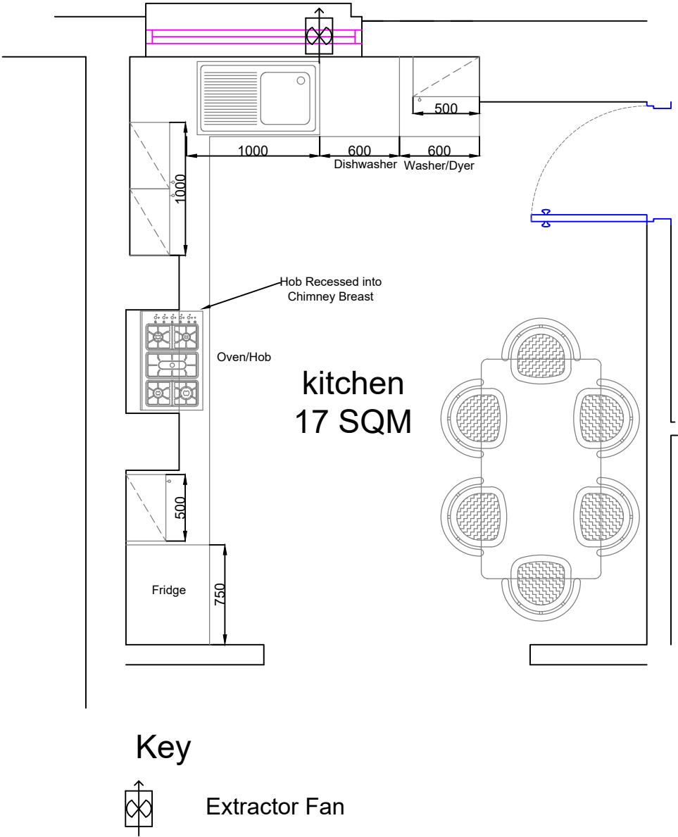
kitchen layout plan
