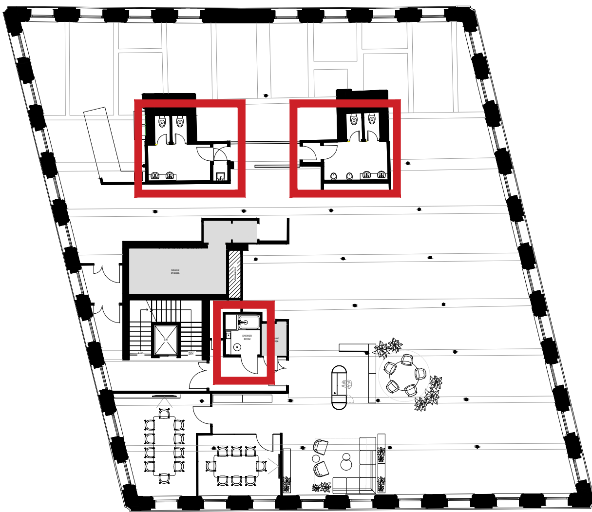
FOURTH FLOOR PLAN 1:200
