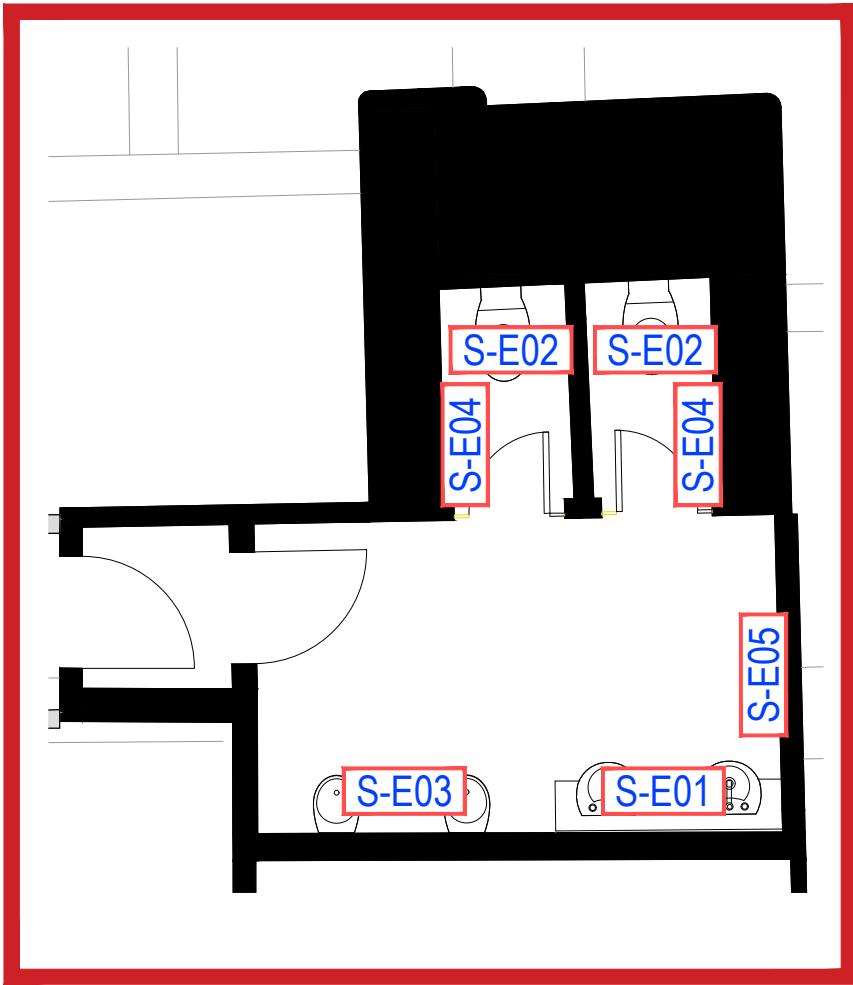
4F MALE WC ZOOM IN 1:50
