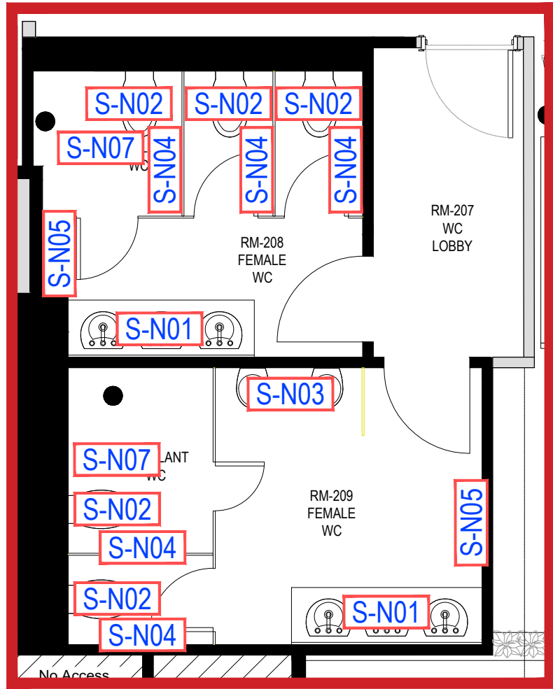
2F WCS ZOOM IN 1:50
