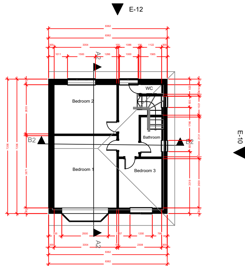
3 Exg First Floor Plan Scale 1:125@A3
