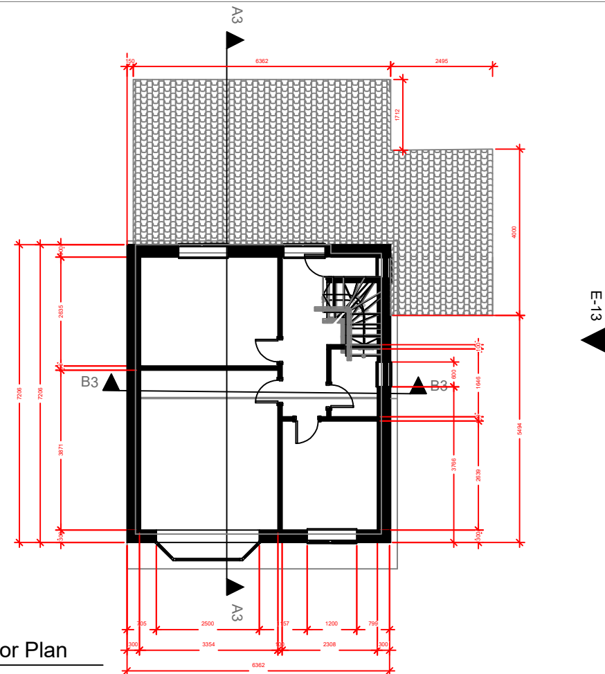
2 Prop Ground Floor Plan Scale 1:125@A3
