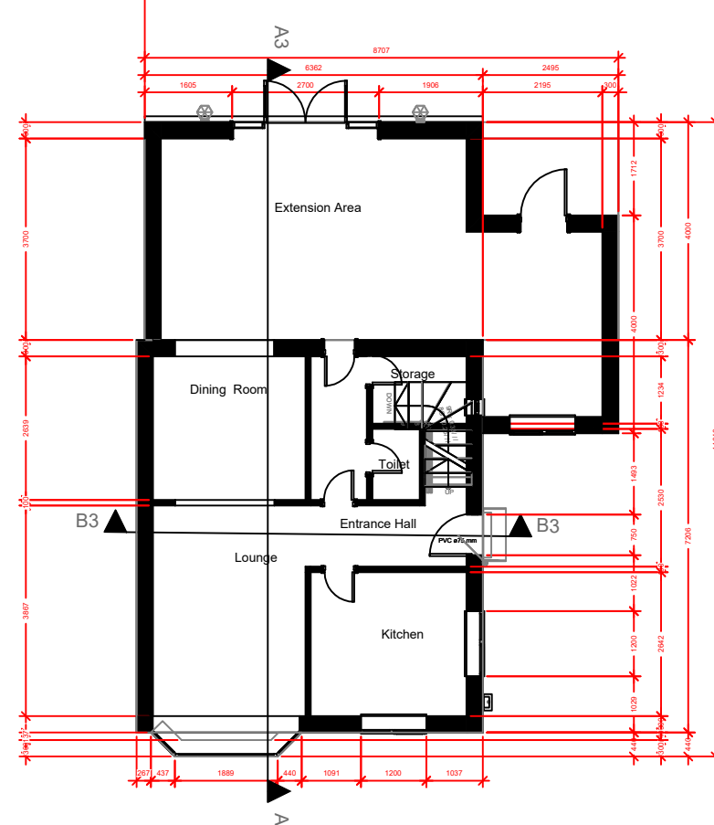
2 Prop Ground Floor Plan Scale 1:125@A3
