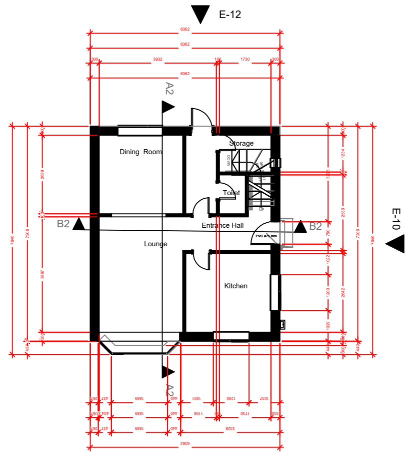
1 Exg Ground Floor Plan Scale 1:125@A3
