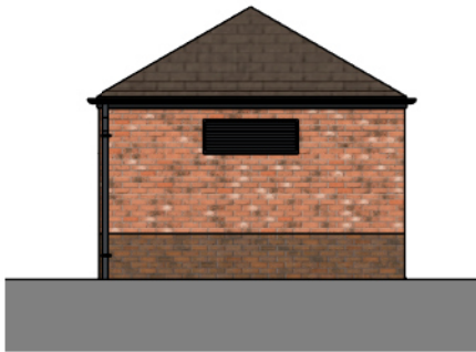
Left Elevation
