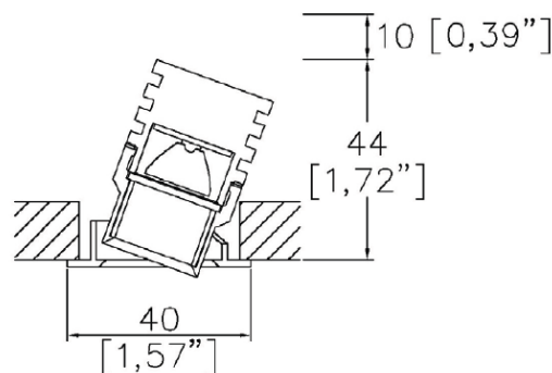
043-FA-TR Cut-out 36mm Ø
