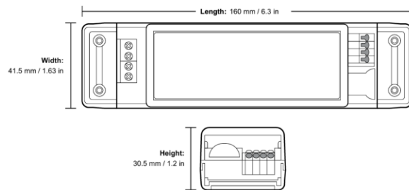
ECodrive 240/A-BIS
