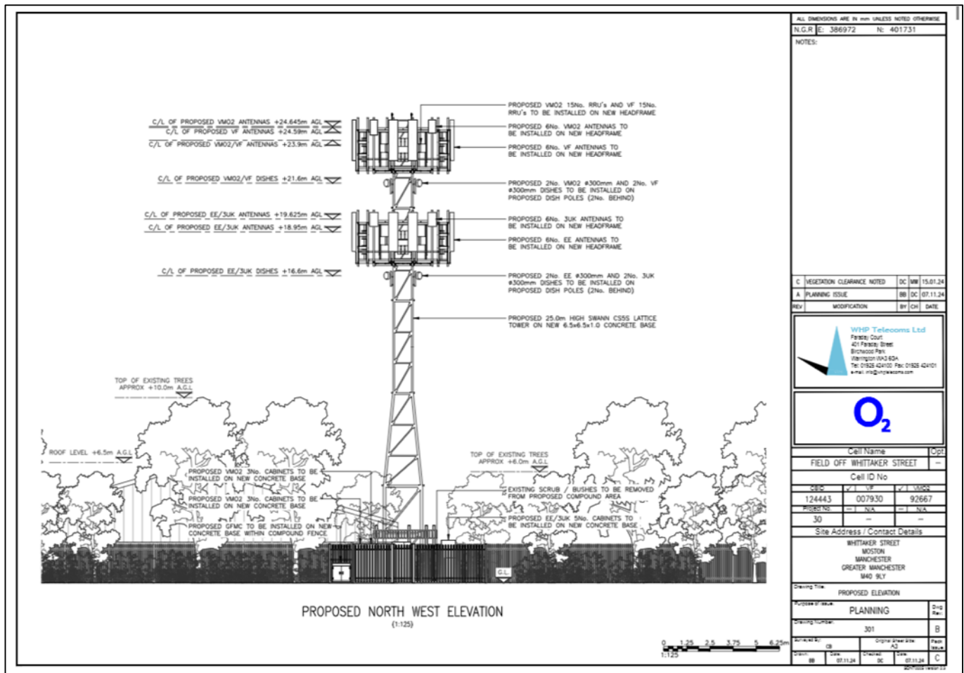
Figure 2. Proposed elevation
