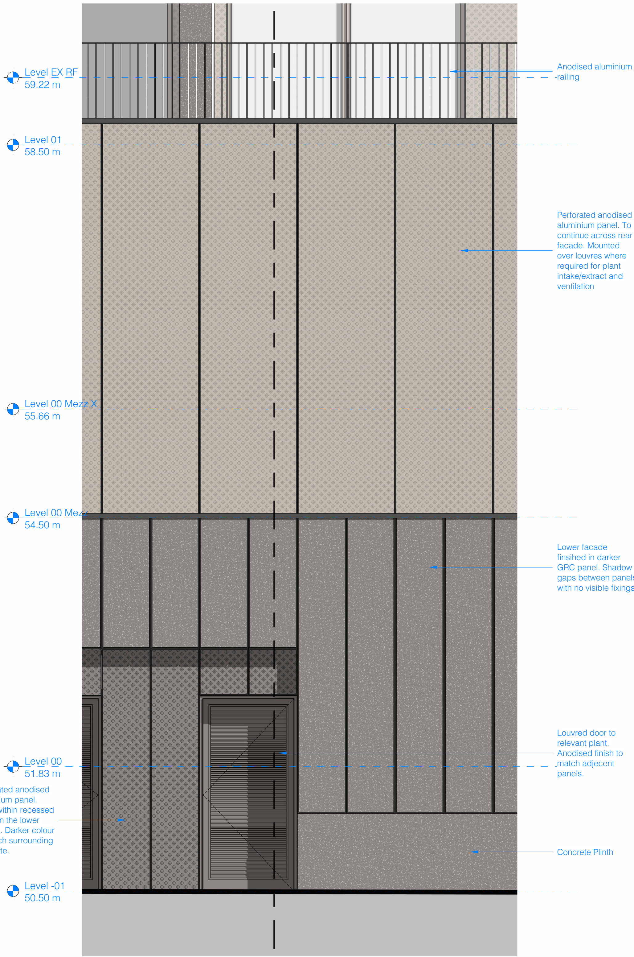
2 Elevation - North West Fragment 1 : 25
