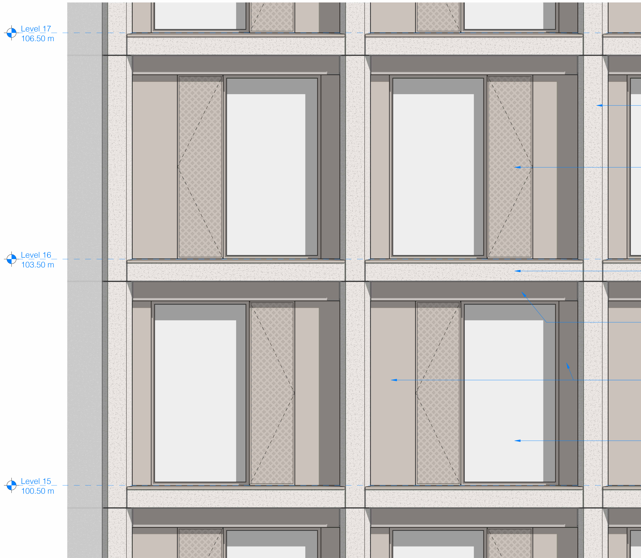
1 Elevation - South East Typical Fragment 1 : 25
