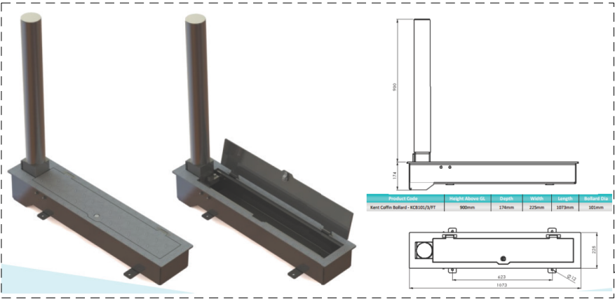
2no. Kent Coffin Bollards – KCB101/3/FT or similar countersunk foldable bollards in front of gates – as stated within drawing CDN230514 by DEP. Kent metallic black finish. 1no reflective strip only if required. To be raised as default and lowered by concierge when necessary.
