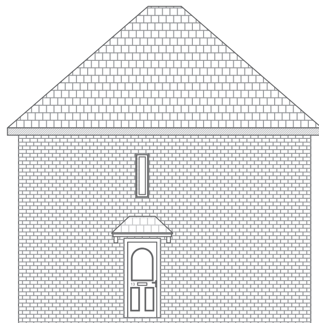
Existing L/H/S elevation
