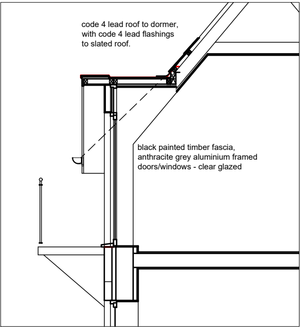
DORMER SECTION 1:50
