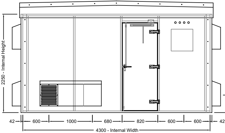
LH SIDE ELEVATION
