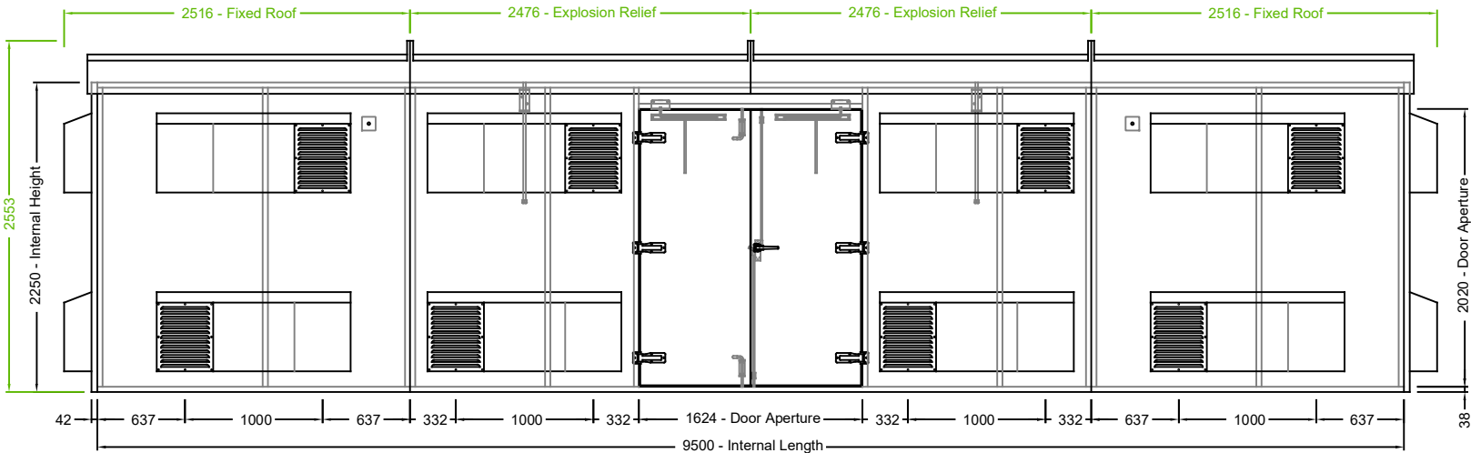
FRONT & REAR ELEVATIONS
