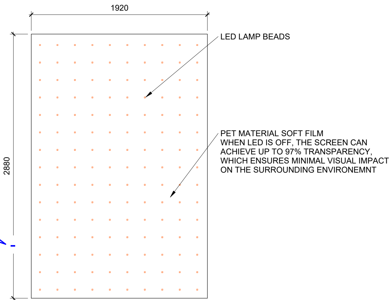
03 INTERNAL LED DISPLAY SOFT FILM 1 : 25
