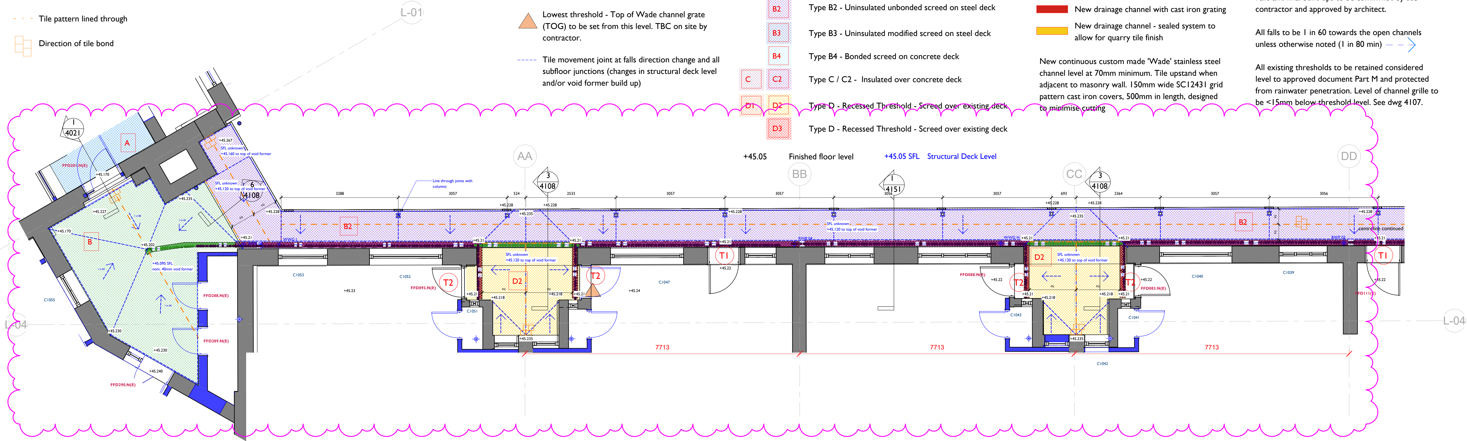
01 First Floor - Fairfield St Walkway East 1 : 50
