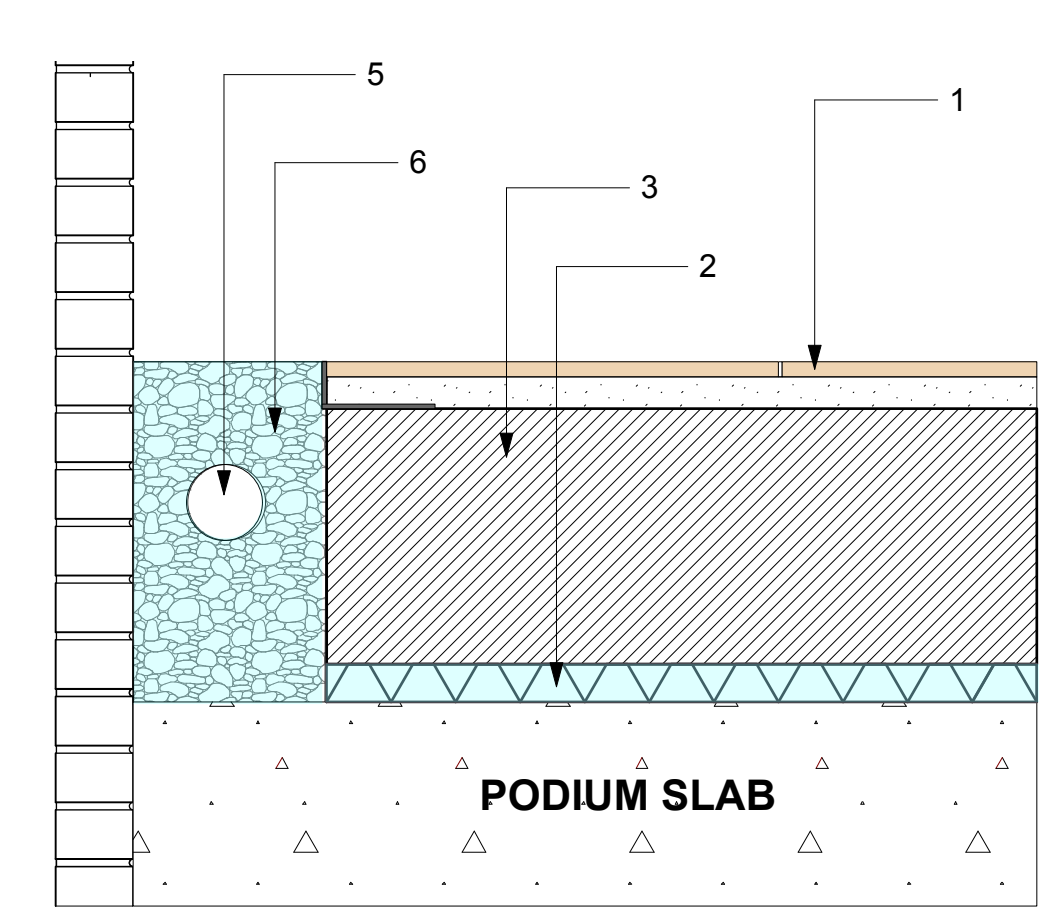
3 Deck Drain/ Gravel Drain on Void Former Scale: 1:10
