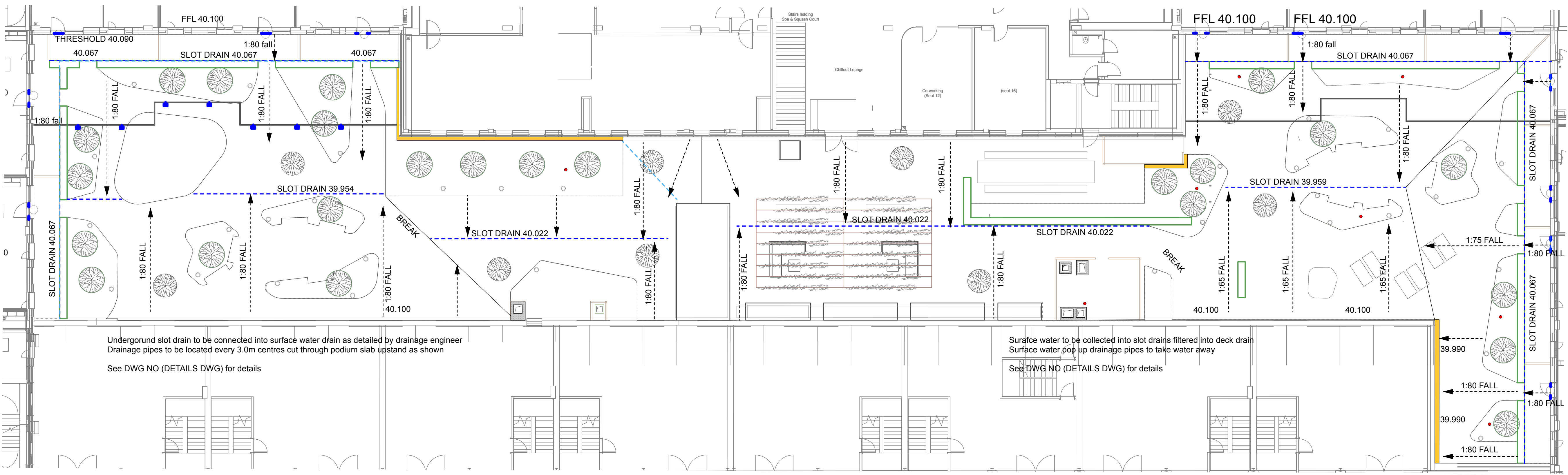
1 Podium Drainage Strategy Scale: 1:150
