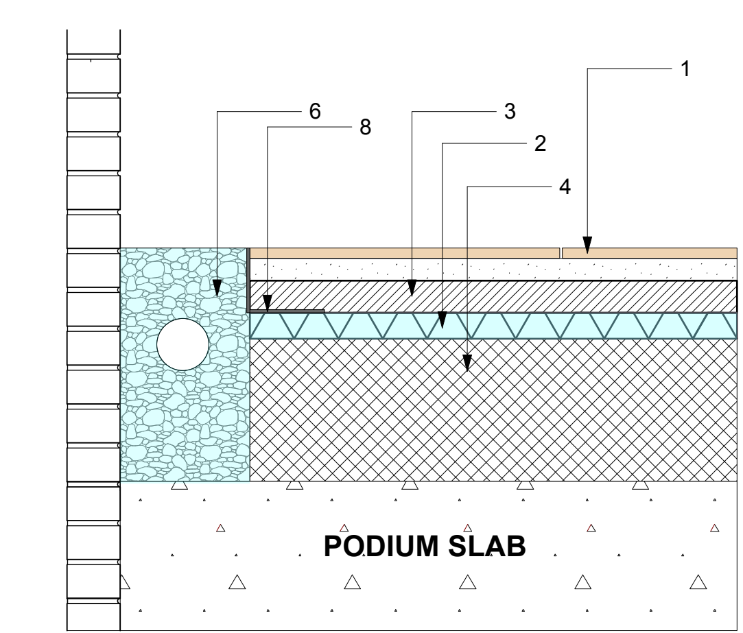
2 Deck Drain /Pebble Drainage -Insulation Scale: 1:10
