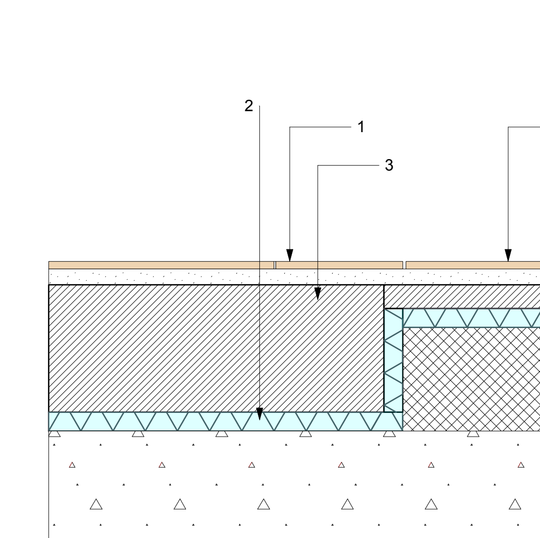
6 Deck Drain transition between Void Fomer & Insulation Scale: 1:10
