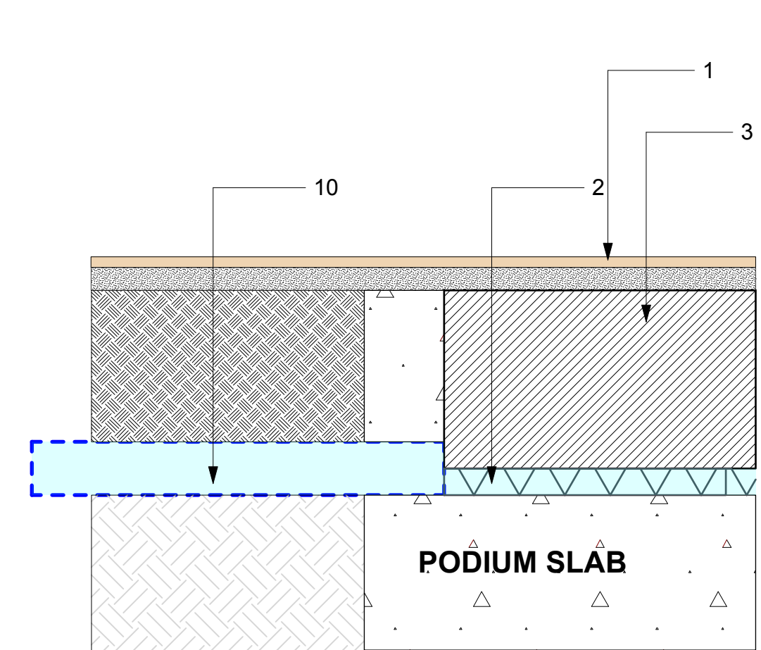
5 Deck Drain to SWP thro Concrete Upstand Scale: 1:10
