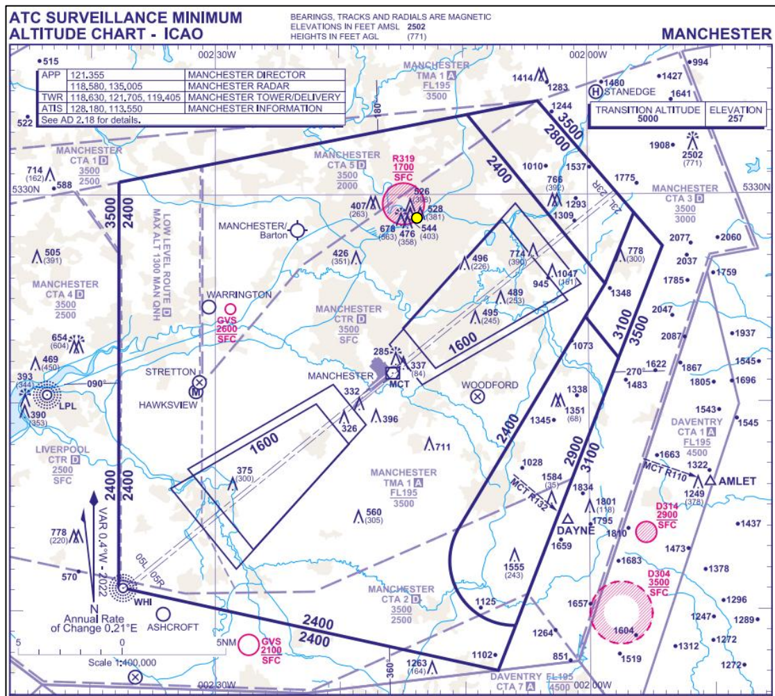
Figure 13 Manchester Airport ATC Surveillance Minimum Altitude Chart
