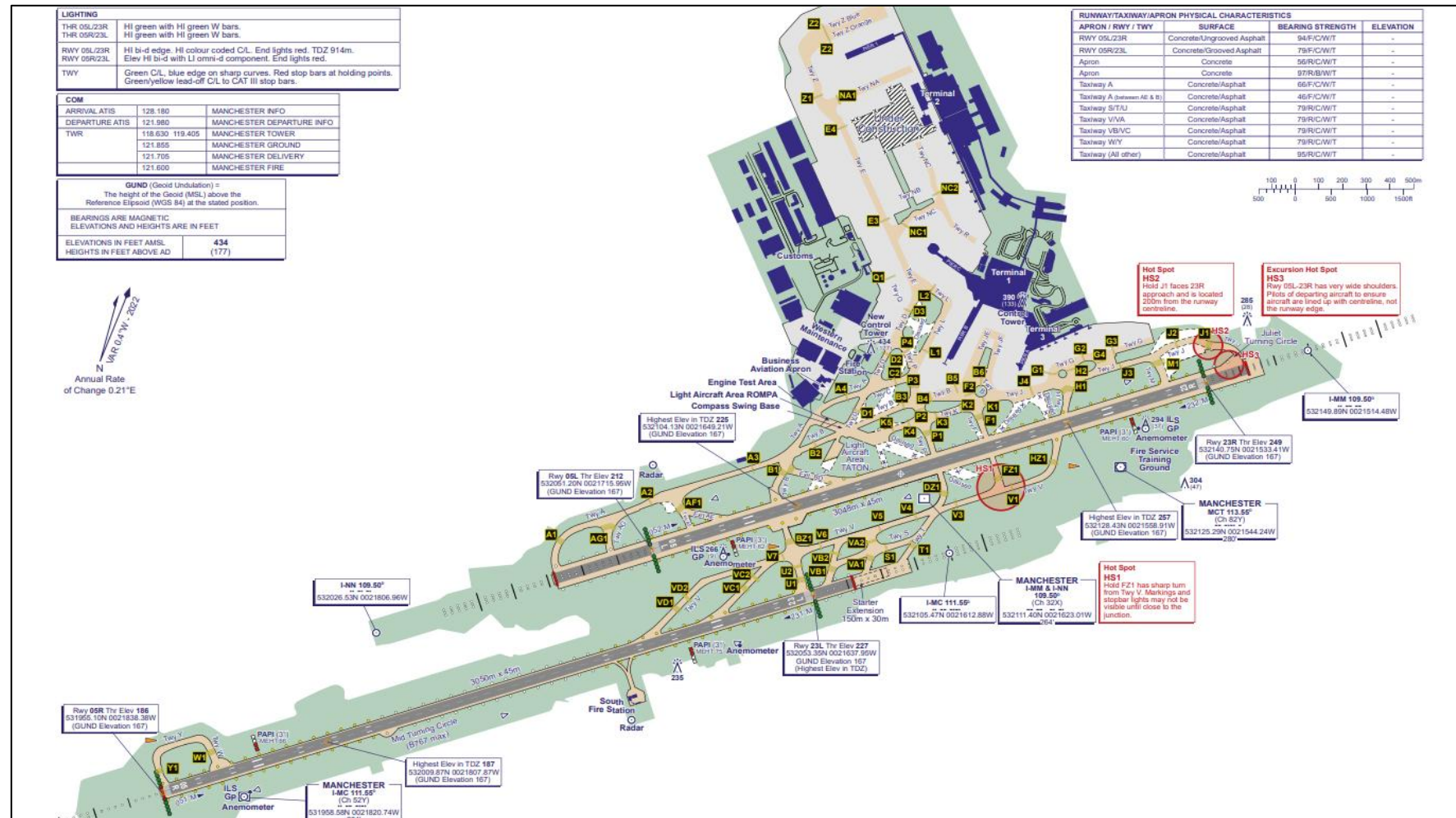
Figure 6 Aerodrome Chart for Manchester Airport
