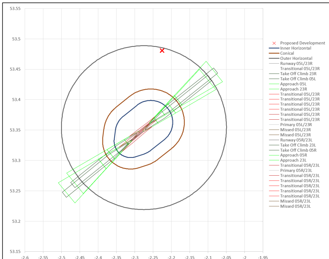
Figure 11 Manchester Airport Obstacle Limitation Surfaces chart
