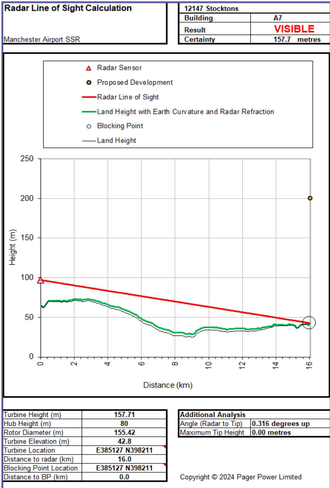
Figure 8 Radar line of sight chart - building point H
