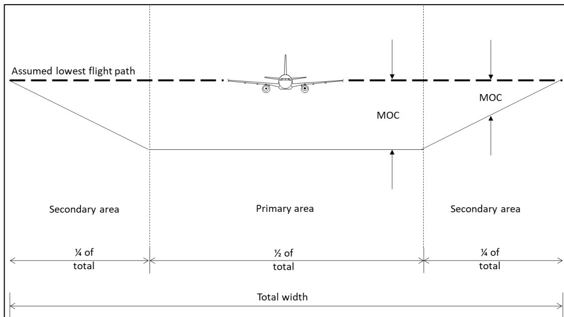
Figure 12 Instrument Flight Procedure Minimum Obstacle Clearances
