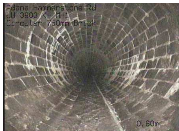
UU 3803X_eca04b50-e131-4dfe-8786-ba9a1bf9edd0_20230929_110618_260.jpg, 00:00:38, 0.60 m Attached deposits, encrustation from 7 o'clock to 5 o'clock, 5% cross-sectional area loss, start, Patchy
