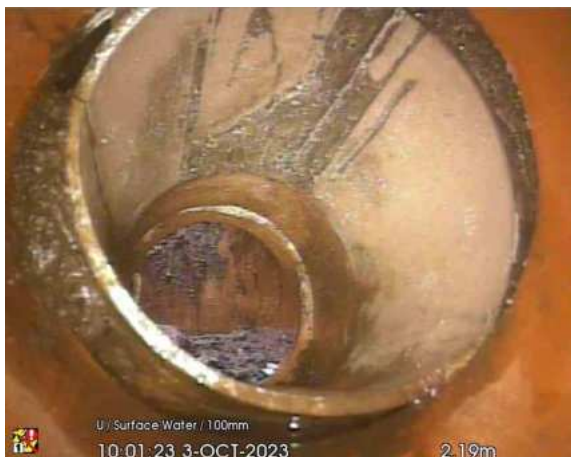
MH18 US GULLY_2-19m_100123.jpg, 00:00:14, 2.19 m Joint displaced, large
