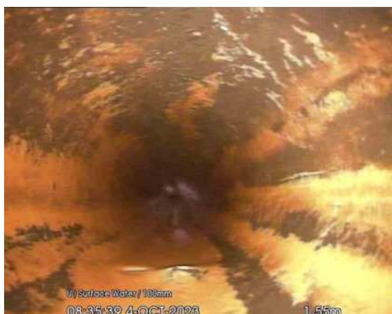
MH3 US RWP_1-55m_083539.jpg, 00:00:12, 1.55 m Deformed sewer or drain, 15%
