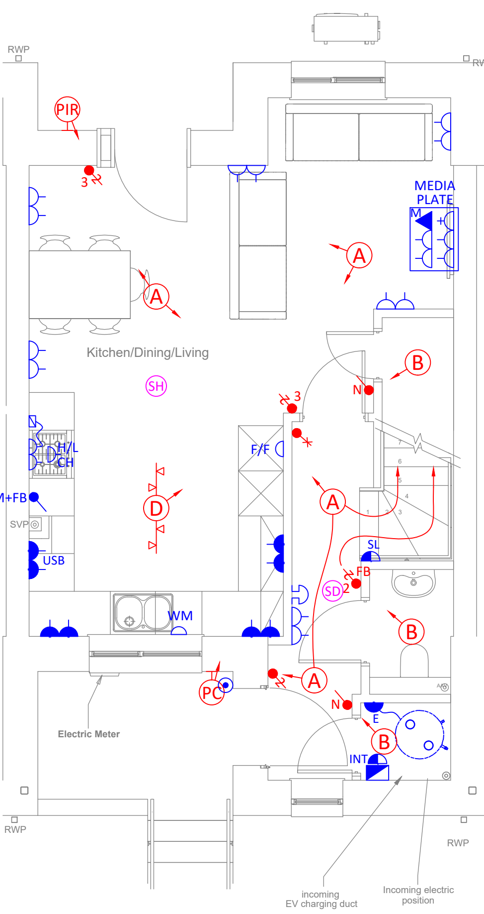
HOUSE TYPE 2 GROUND FLOOR
