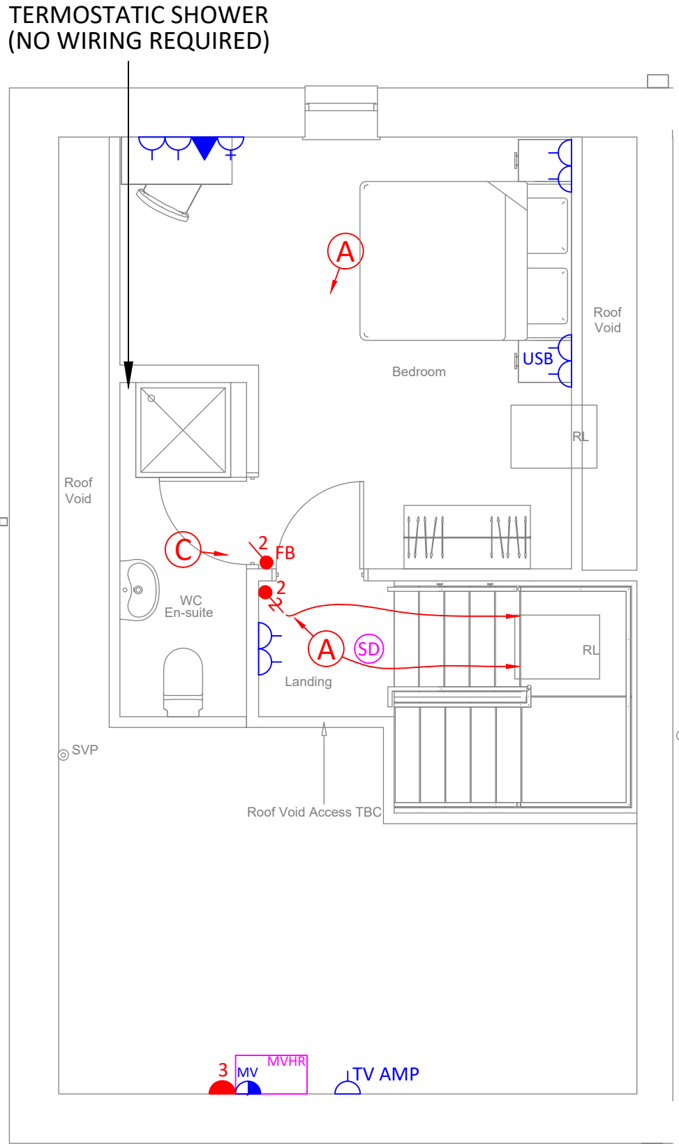
SECOND FLOOR
