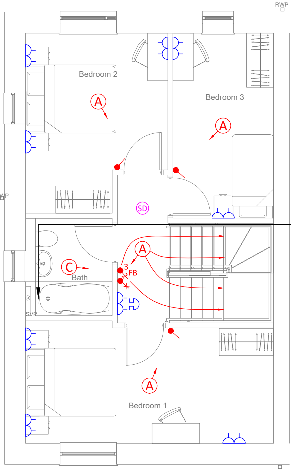
FIRST FLOOR
