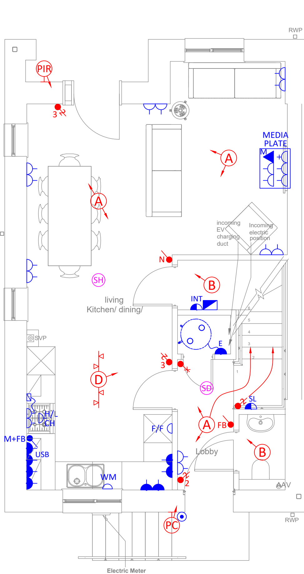
HOUSE TYPE 1 GROUND FLOOR
