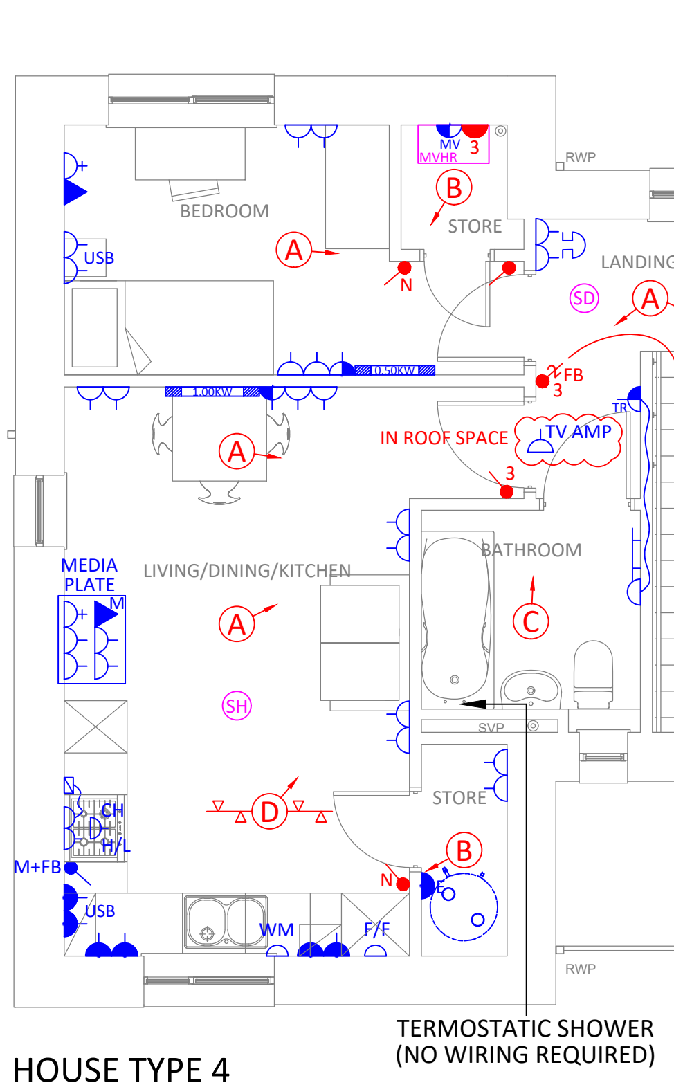
HOUSE TYPE 4 FIRST FLOOR
