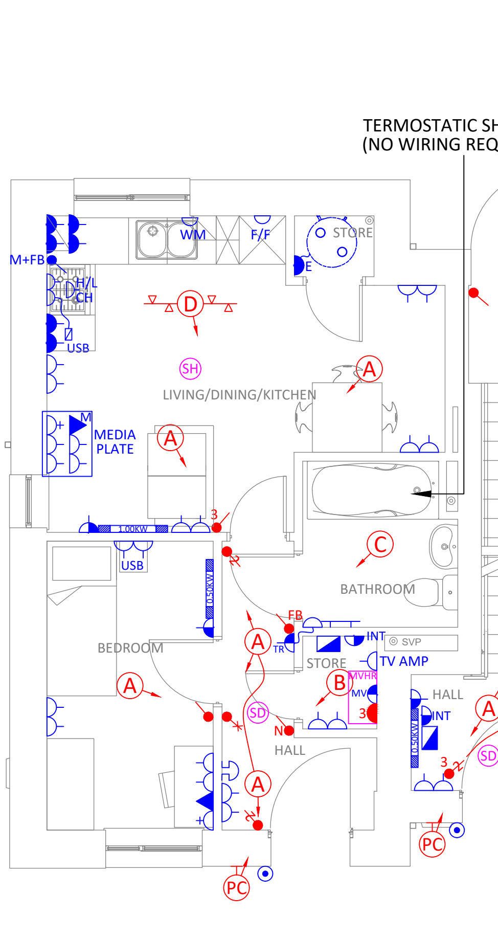
HOUSE TYPE 3 GROUND FLOOR
