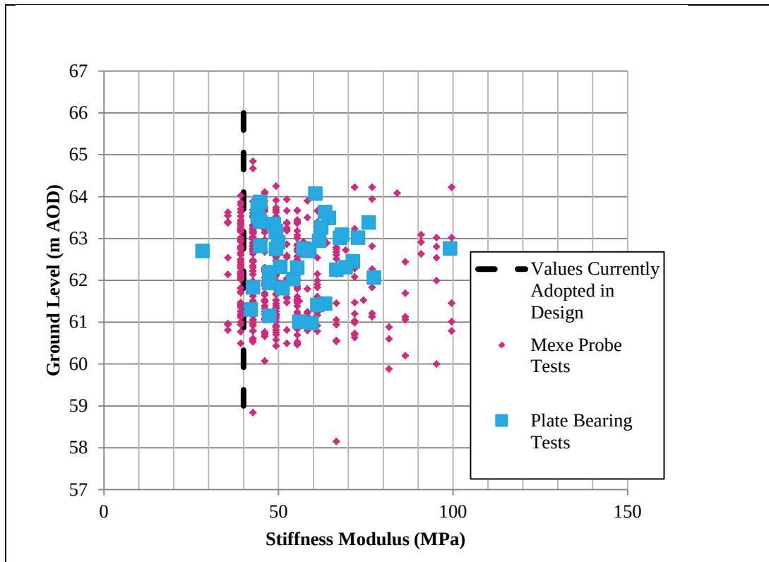
Figure 10 Assessment of Stiffness Modulus E_u for General Engineered Fill below Energy Centre based on field tests.
