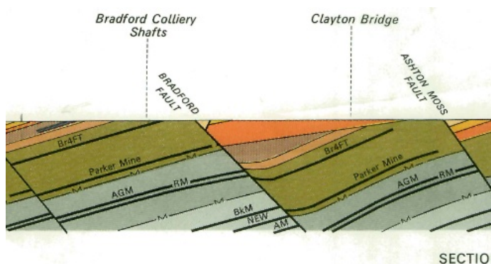
Figure 5 Geological Map extract showing Bradford Fault (section of west to east orientation)
