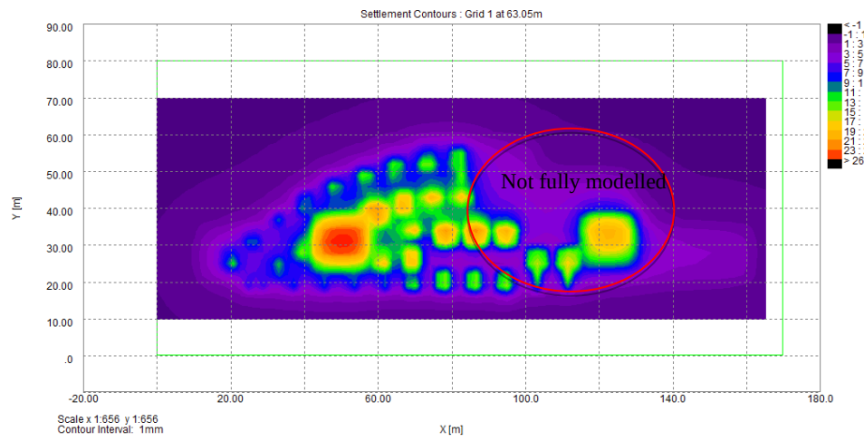
Figure 27 Run 2 Elite Building Settlement Contours at 63.05mOD Ground Floor Slab Formation –case: pool full, DL + ave. LL for core pads
