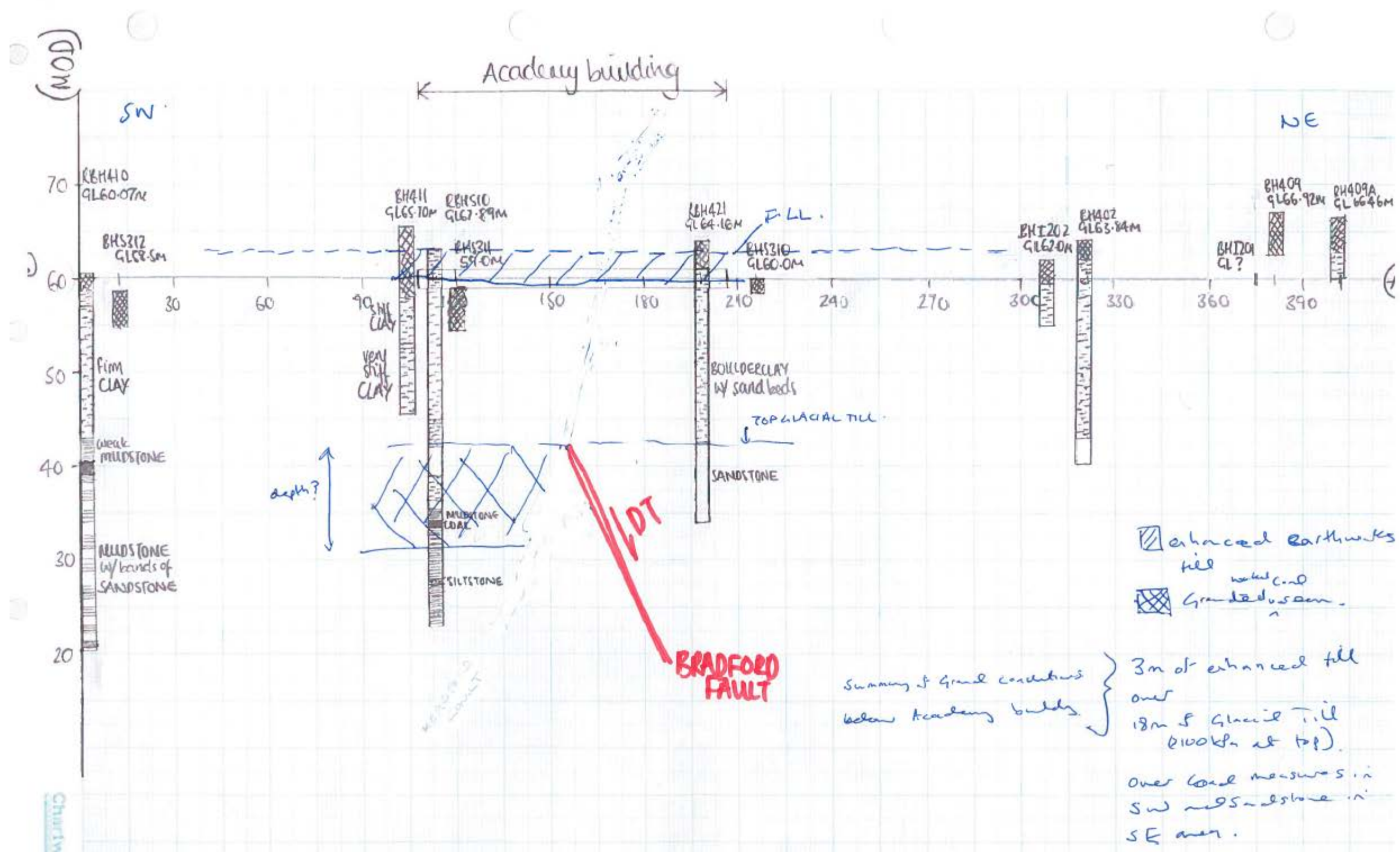
Figure 6 Indicative Geological Cross Section through Academy Building (Section looking to the North West i.e. Section line SW to NE)
