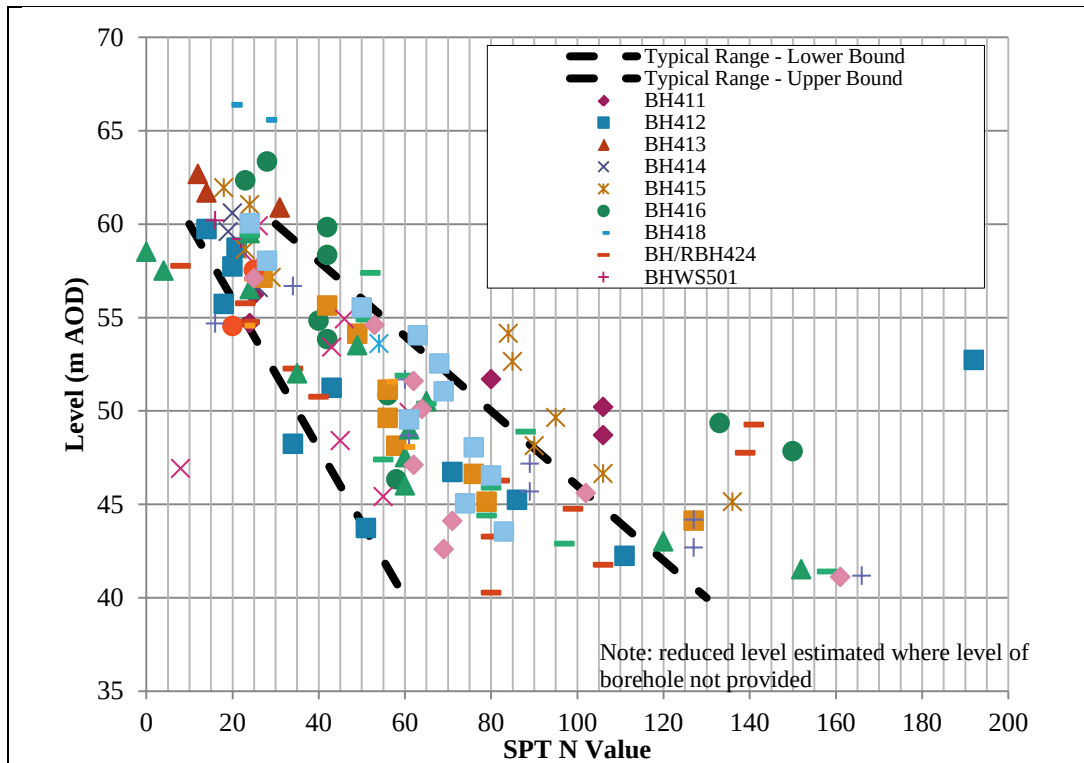
Figure 15 Site wide SPT vs. Reduced Level Plot for Glacial Till
