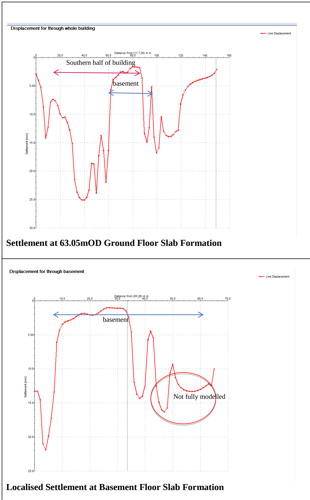
Figure 26 Run 1 Elite Building Settlement –case: pool empty, DL + ave. LL for core pads
