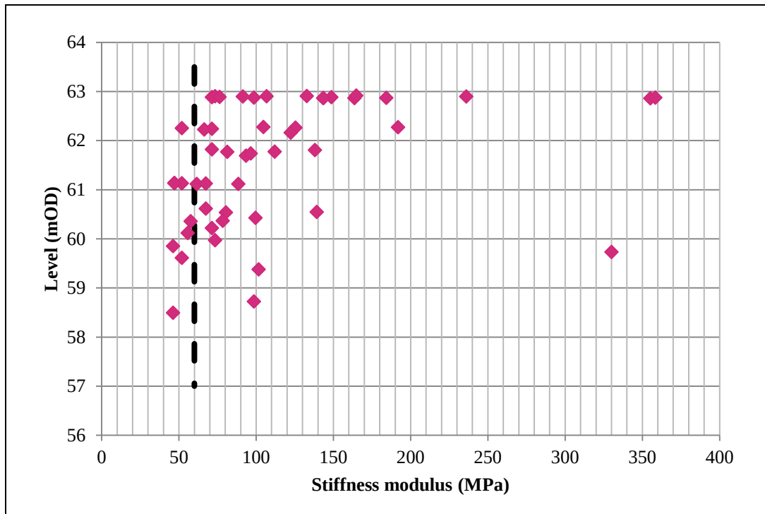
Figure 13 Assessment of Stiffness Modulus E' for Enhanced Engineered Fill below Academy Building from field tests
