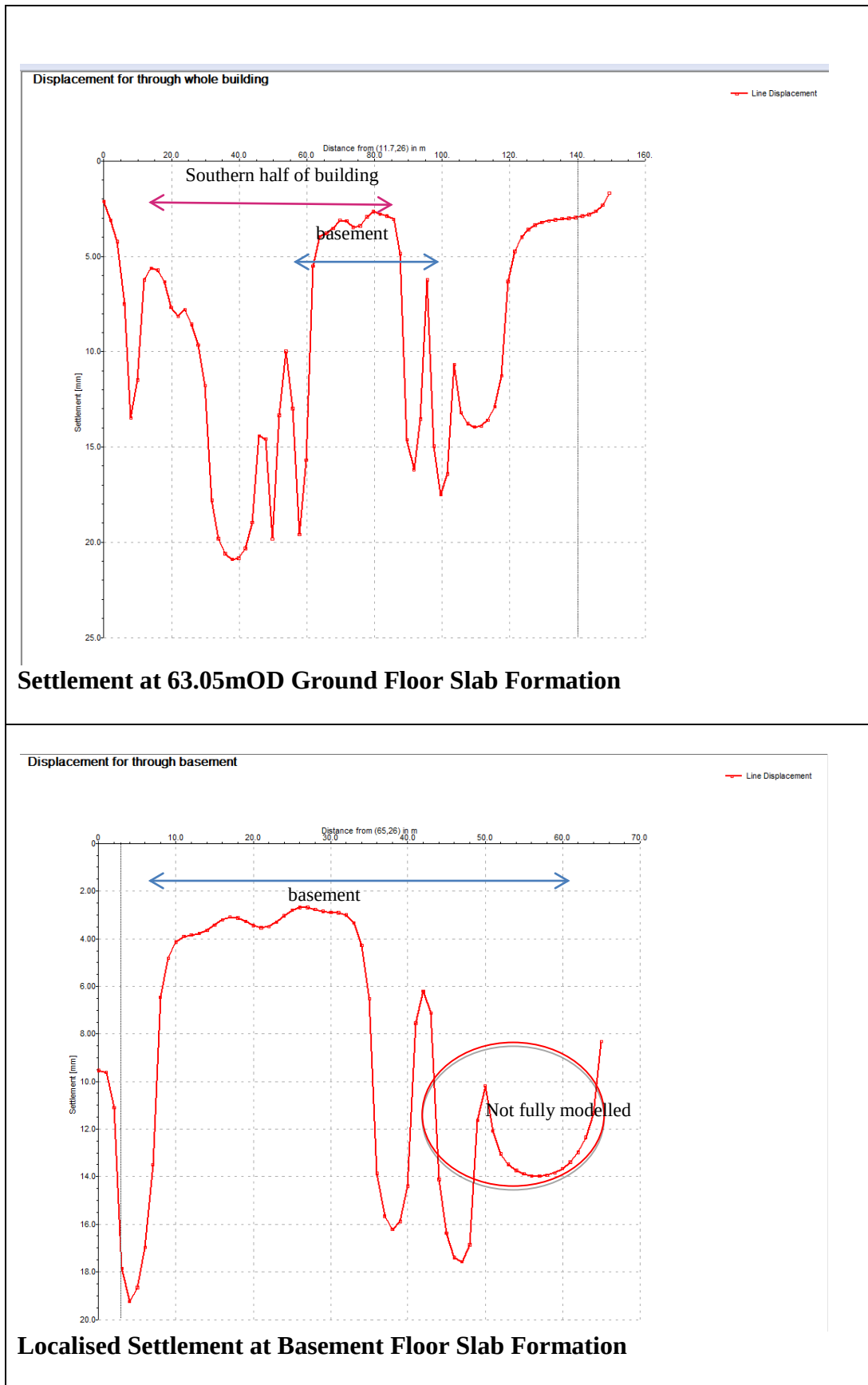
Figure 28 Run 2 Elite Building Settlement –case: pool full, DL + ave. LL for core pads
