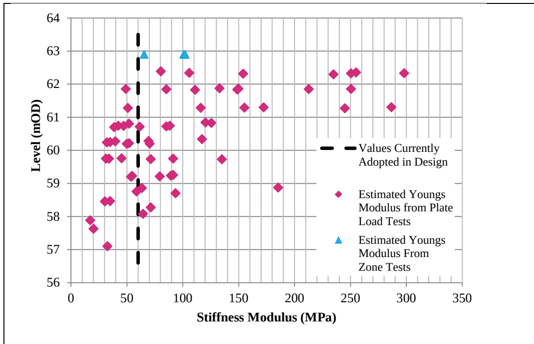
Figure 12 Assessment of Stiffness Modulus E' for Enhanced Engineered Fill below Elite Building from field tests
