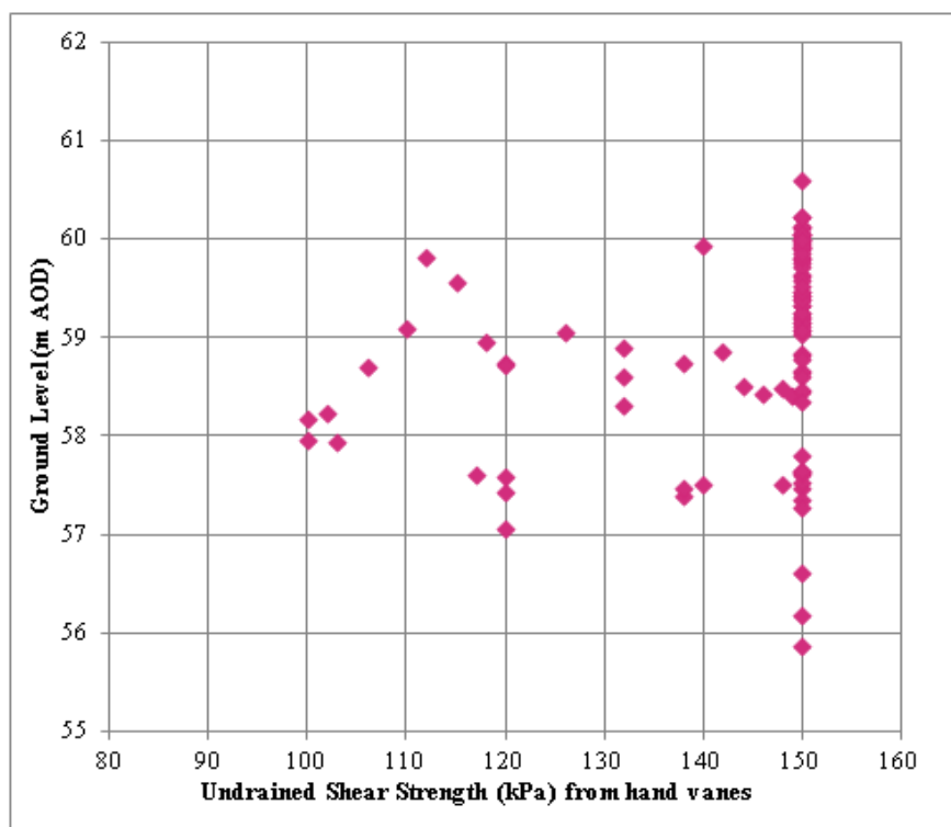
Figure 14 Undrained Shear Strength ( C_u in kPa) at top of Glacial Till (rolled base of excavation in enhanced earthworks area)
