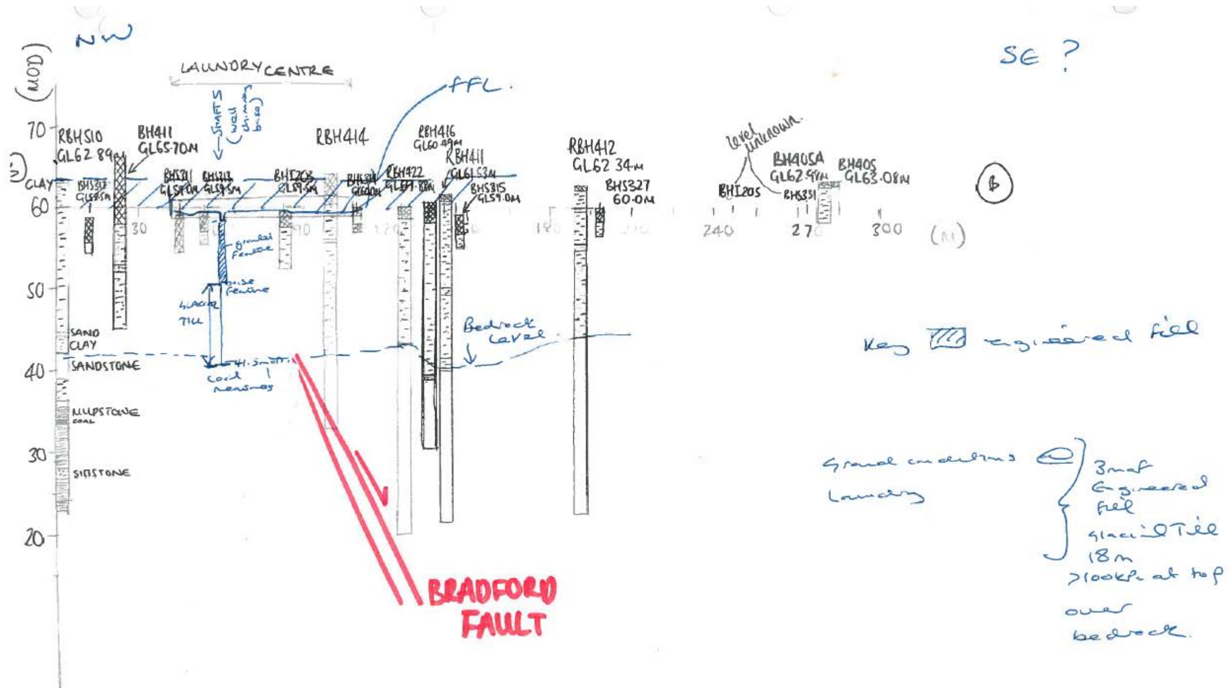
Figure 9 Indicative Geological Cross Section through southern CTF i.e. former Laundry Centre (Section looking to North East i.e. Section line NW to SE)
