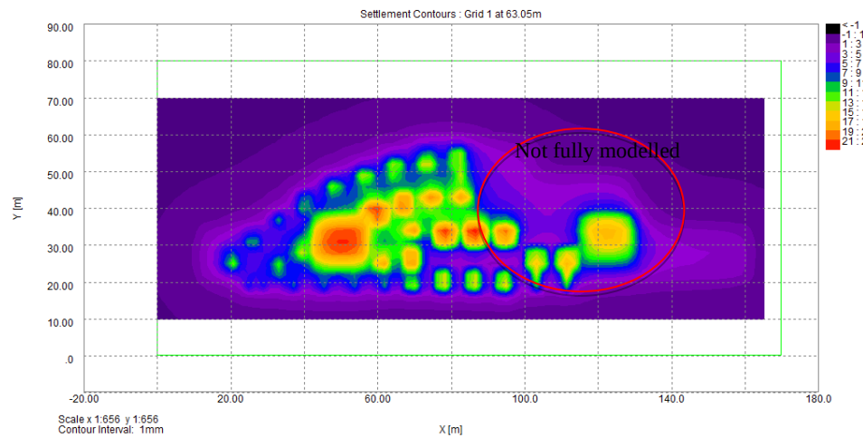
Figure 29 Run 3 Elite Building Settlement Contours at 63.05mOD Ground Floor Slab Formation –case: pool full, DL only for core pads
