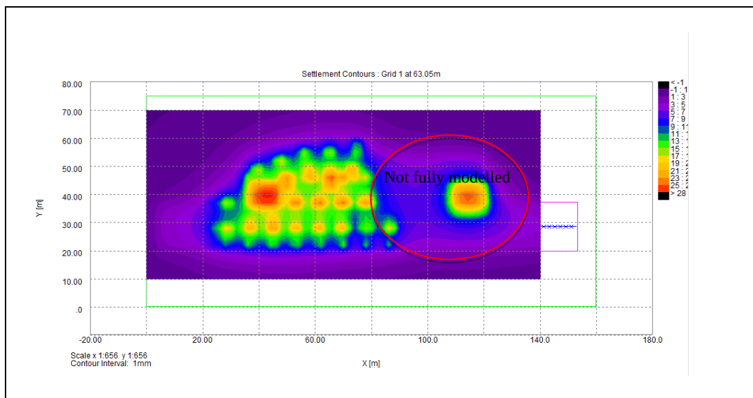
Figure 19 Run 1 Academy Building Settlement Contours at 63.05mOD Ground Floor Slab Formation –case: pool empty, DL + ave. LL for core pads
