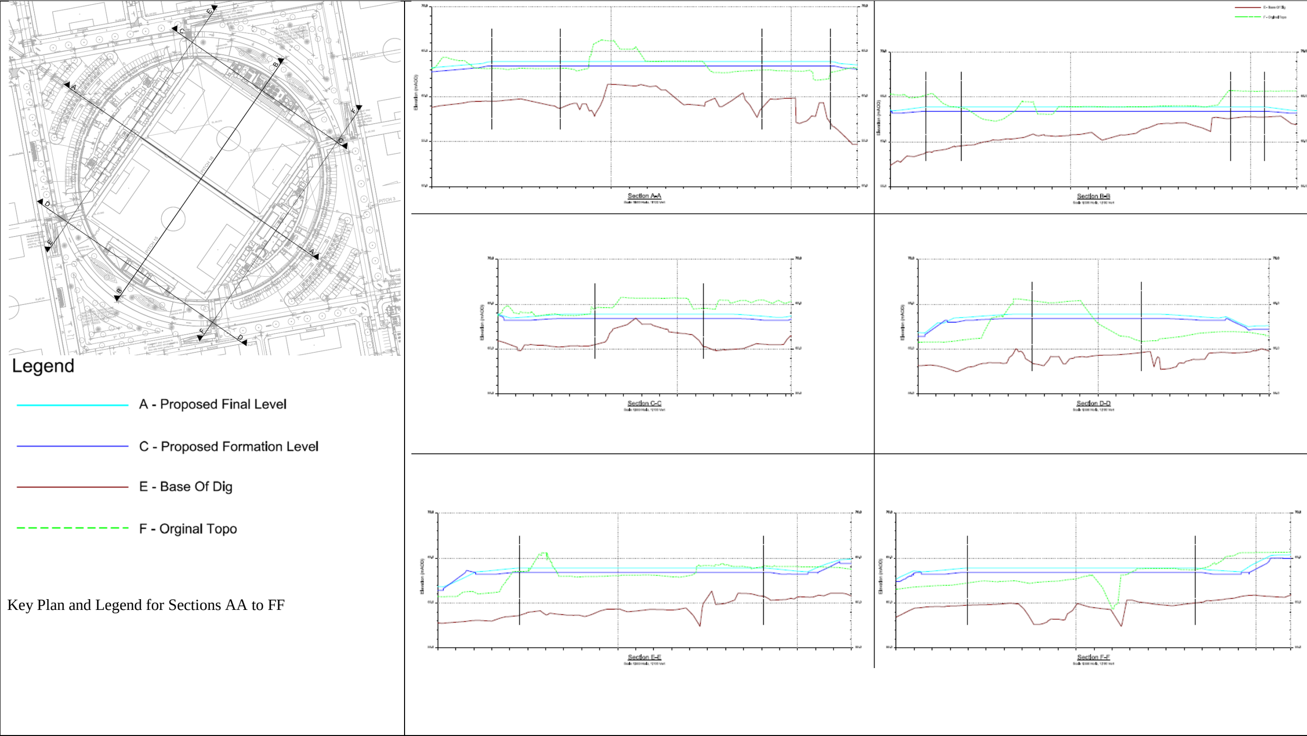
Figure 4 Earthworks Cross Sections for CTF Area (Sections AA to FF)
