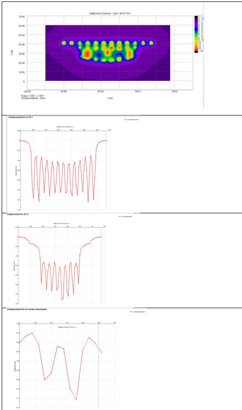
Figure 33: PDISP Run 2 outputs
