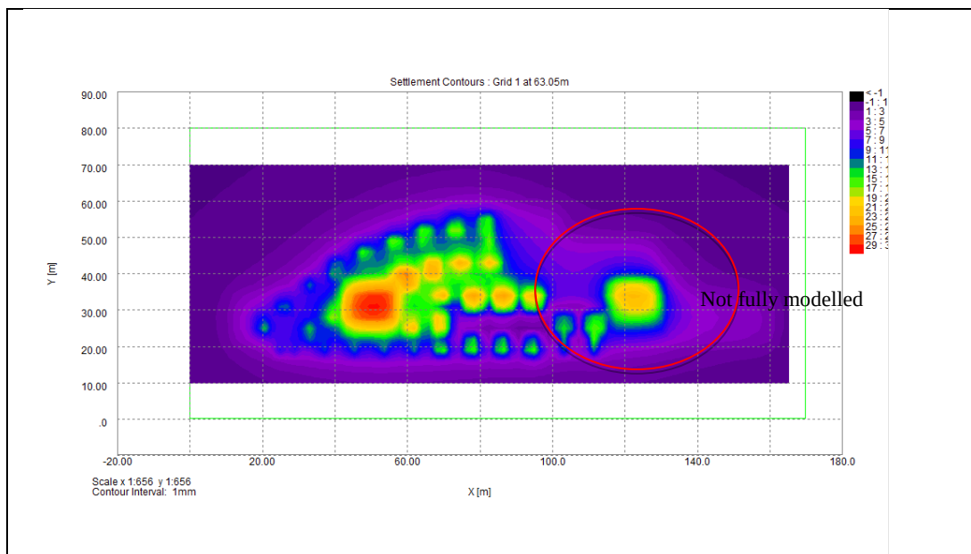
Figure 25 Run 1 Elite Building Settlement Contours at 63.05mOD Ground Floor Slab Formation –case: pool empty, DL + ave. LL for core pads
