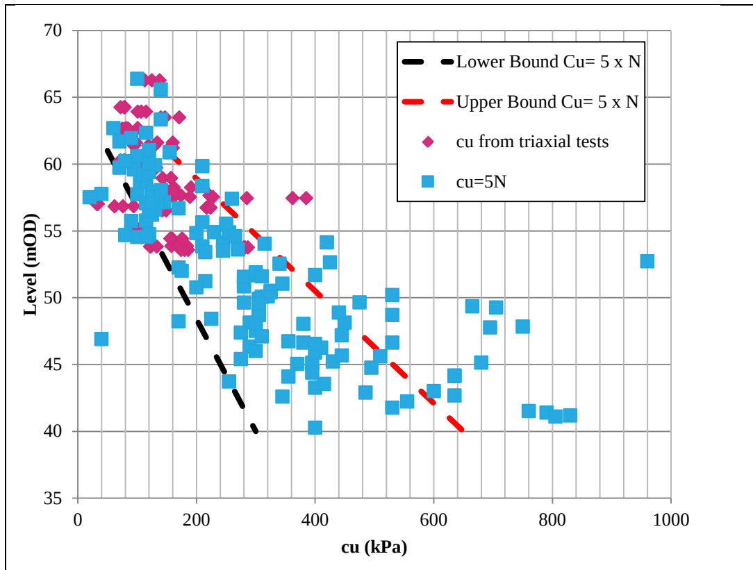
Figure 16 Undrained shear strength, c_u vs. Reduced Level from site wide results
