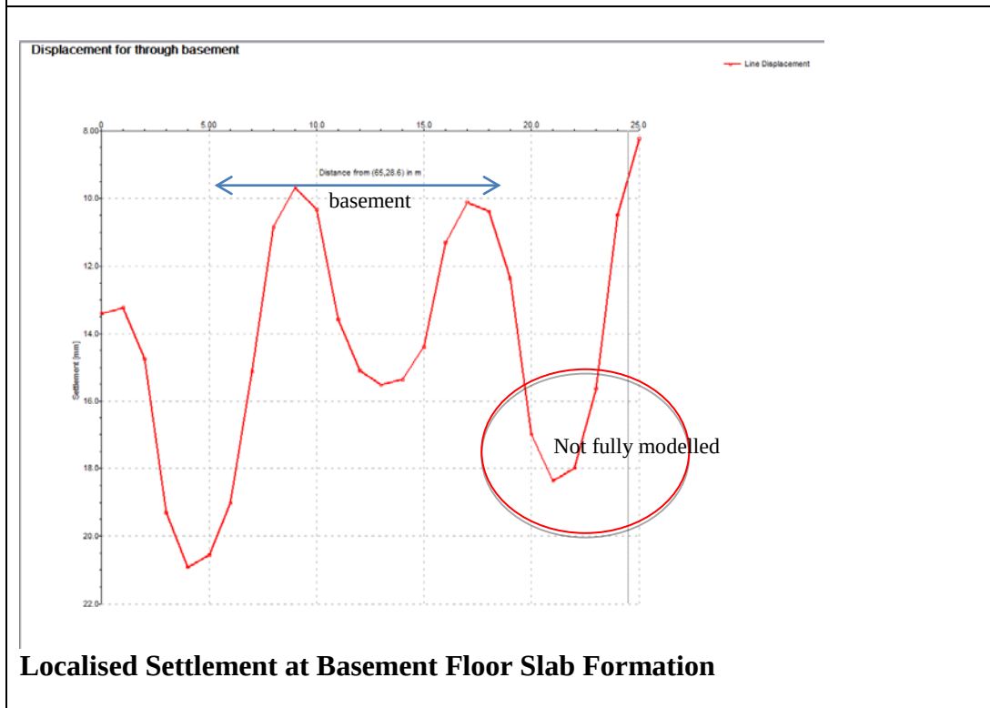
Figure 20 Run 1 Academy Building Settlement –case: pool empty, DL + ave. LL for core pads
