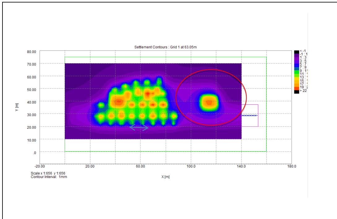
Figure 23 Run 3 Academy Building Settlement Contours at 63.05mOD Ground Floor Slab Formation –case: pool full, DL only for core pads
