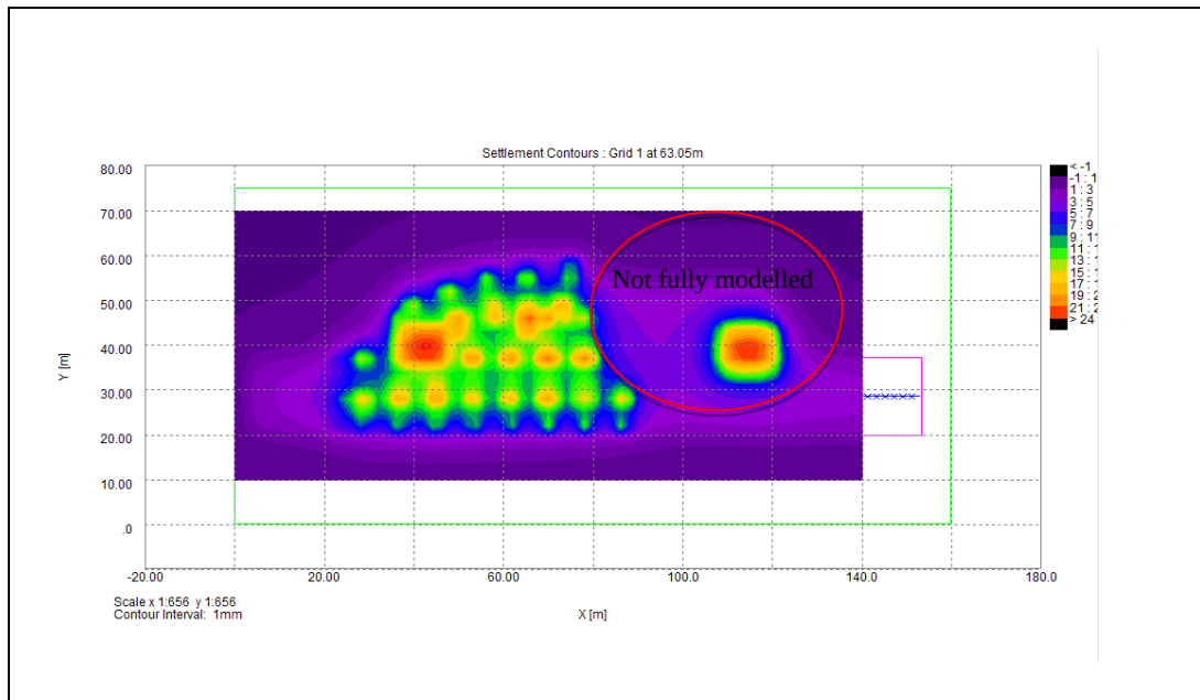
Figure 21 Run 2 Academy Building Settlement Contours at 63.05mOD Ground Floor Slab Formation –case: pool full, DL + ave. LL for core pads
