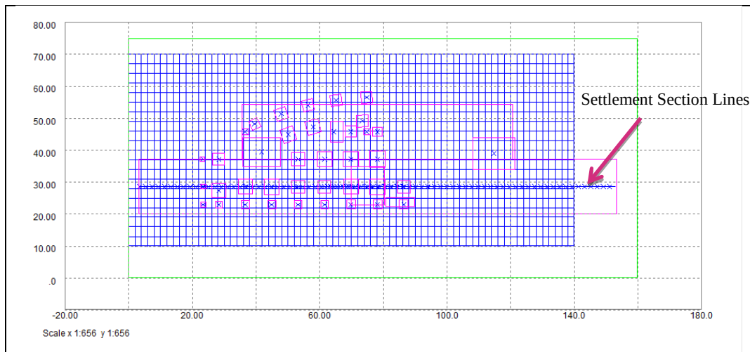
Figure 18: Academy Building PDisp Model Layout (southern half pads considered only)
