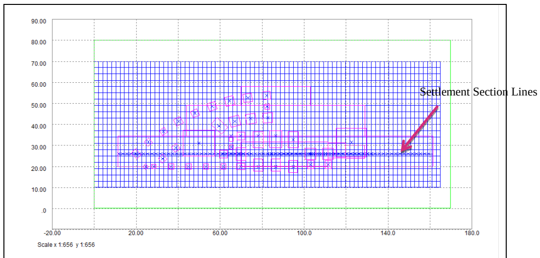
Figure 24 Elite Building Model PDisp Layouts (Northern Half pads considered only)
