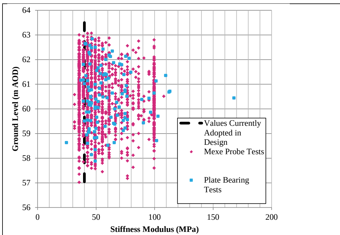
Figure 11 Assessment of Stiffness Modulus E_u for General Engineered Fill below southern CTF (former Laundry Building) based on field tests
