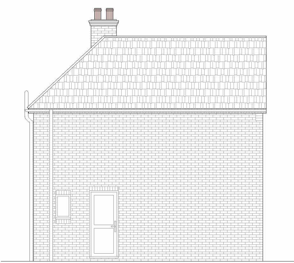
EXISTING SIDE ELEVATION-2
