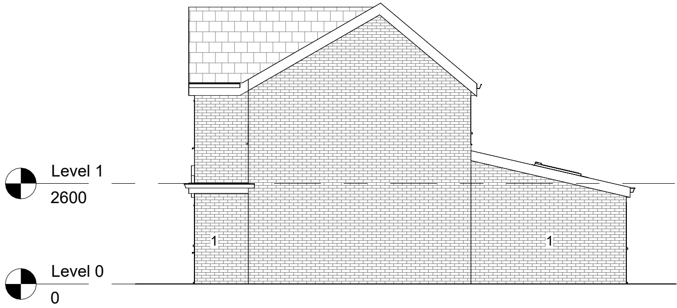
5 SIDE ELEVATION 1 1 : 100
