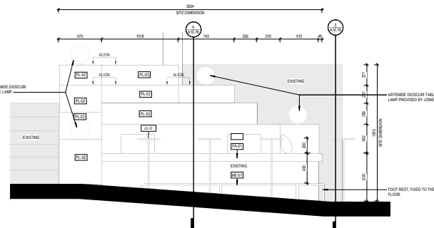
2 JO-11A - ELEVATION 1 - STAIR JOINERY 1:20
