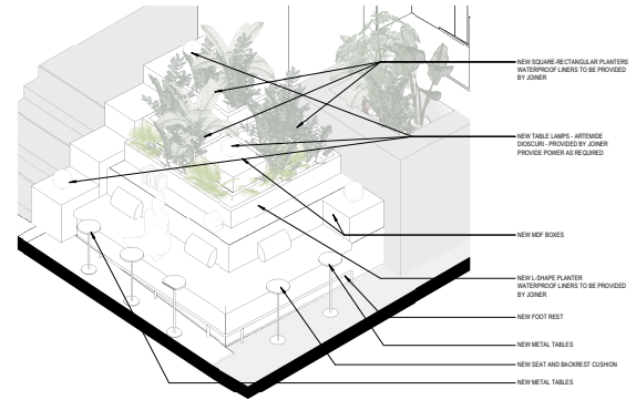
5 JO-11/12 AXONOMETRIC VIEW 1:20
