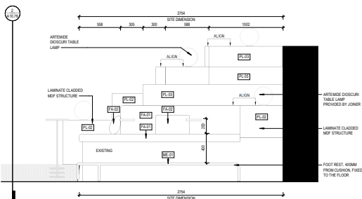
3 JO-11A - ELEVATION 2 - STAIR JOINERY 1:20
