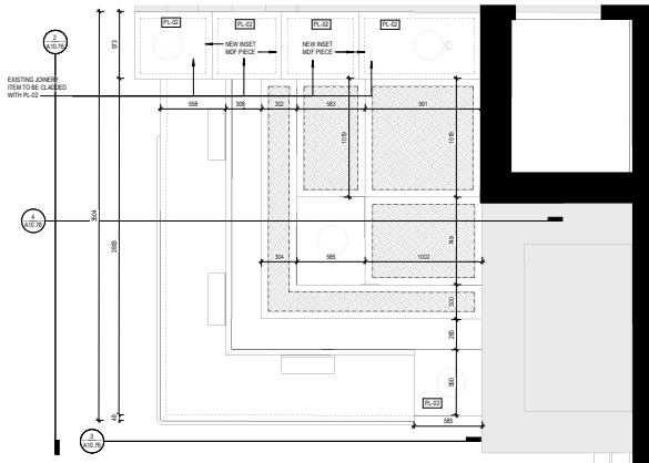
1 JO-11A - PLAN DETAIL - STAIR JOINERY 1:20
