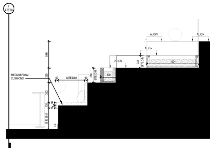
1 JO-11A - SECTION - STAIR JOINERY 1:20
