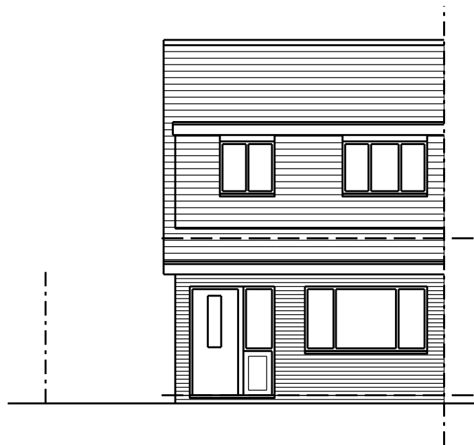
East Elevation
