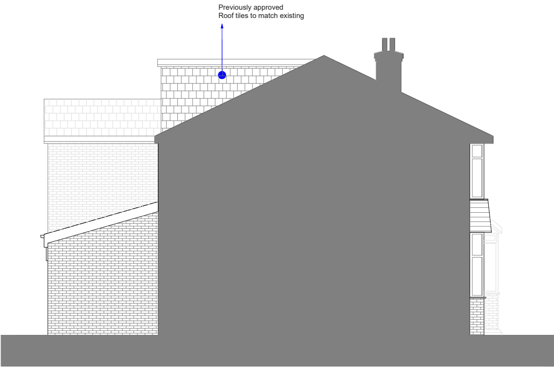
Approved Side Elevation 1:100 A3 0m 1m 3m 5m
