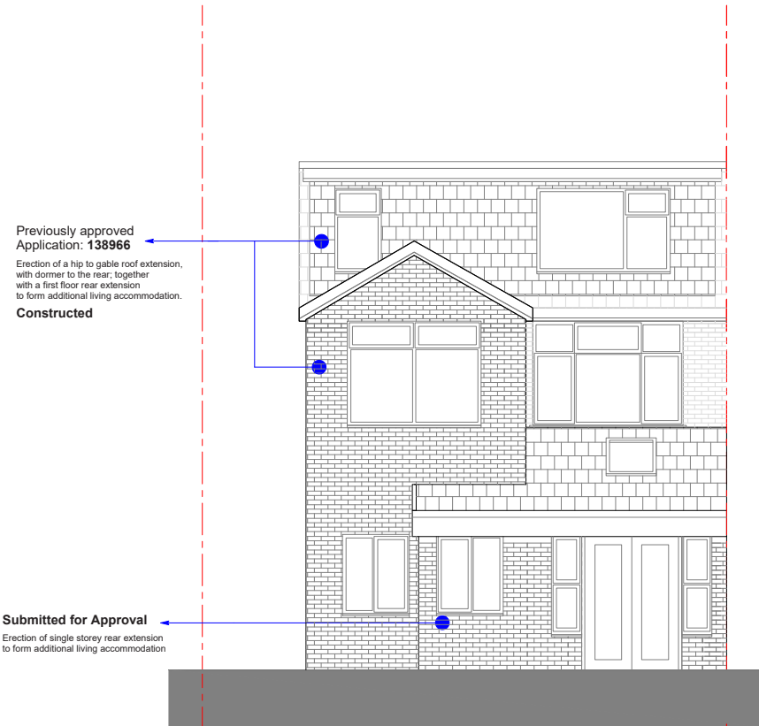
Proposed Rear Elevation 1:100 A3 0m 1m 3m 5m
