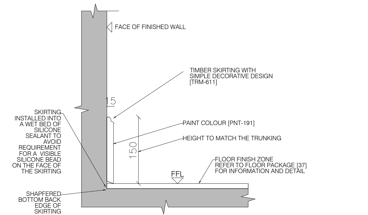
03 INTERNAL SKIRTING - TYPE 1 ON FLOOR FINISH
