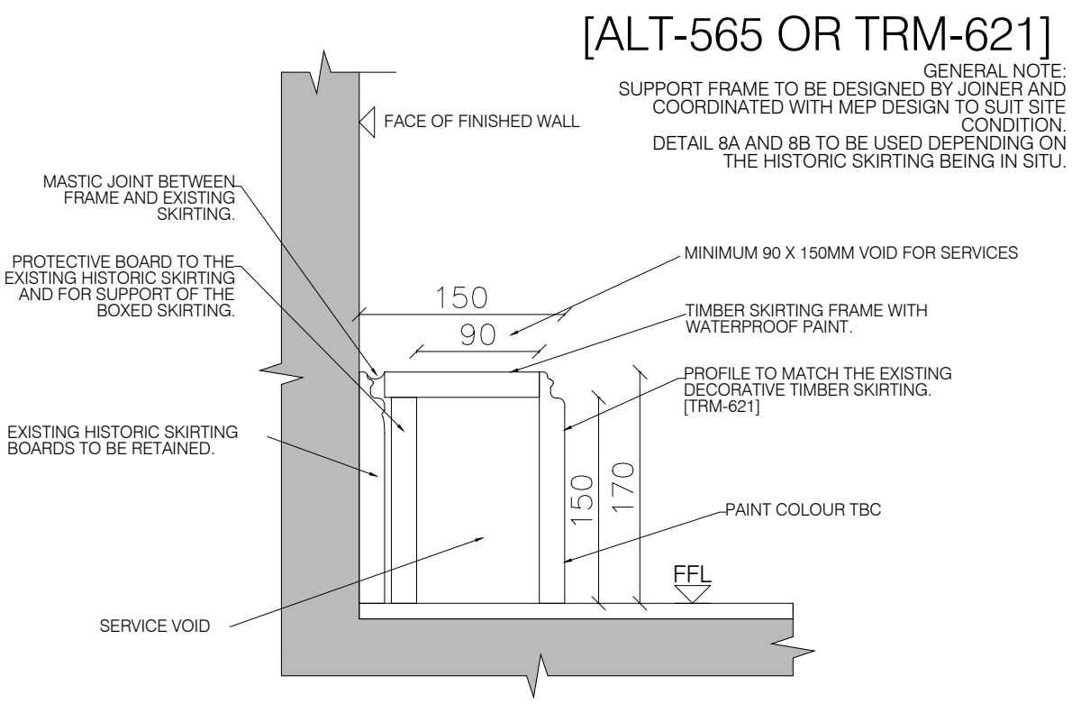
08B INTERNAL SKIRTING - TIMBER WITH SERVICES
