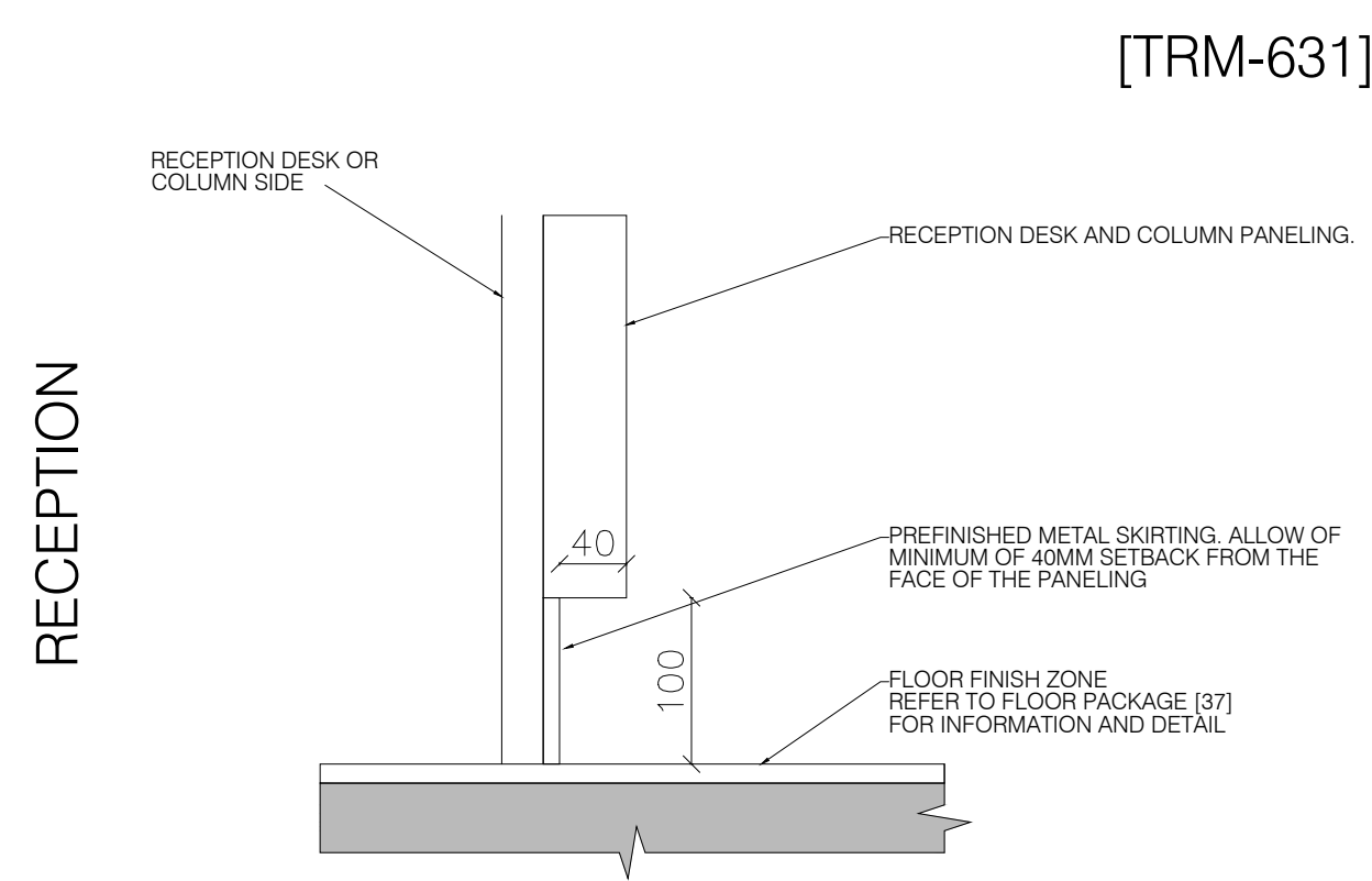
06 INTERNAL METAL SKIRTING DETAIL
