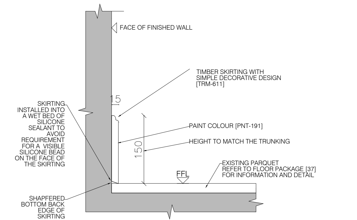
04 INTERNAL SKIRTING - TYPE 1 ON PARQUET
