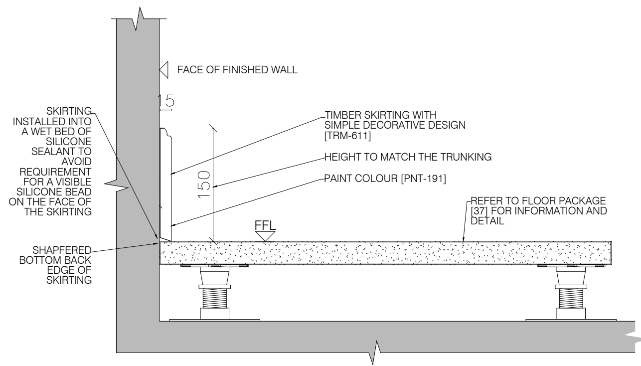
02 INTERNAL SKIRTING DETAIL - TYPE 1 ON RAF
