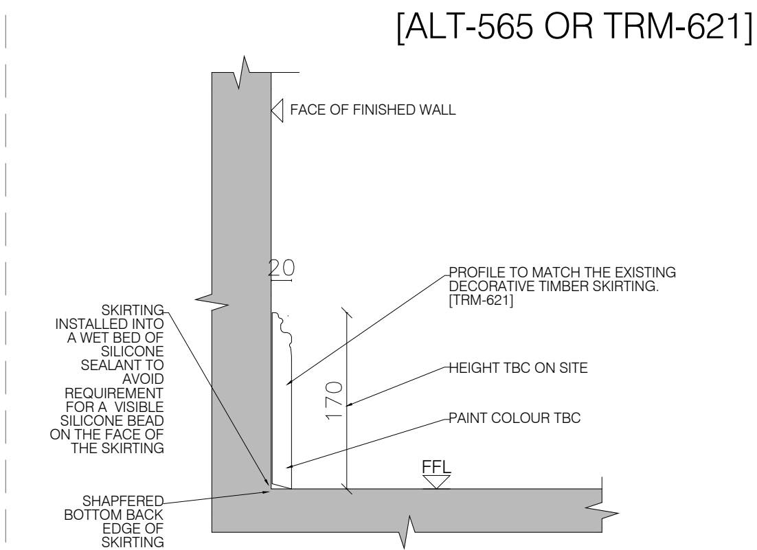
05 INTERNAL SKIRTING DETAIL - TYPE 2
