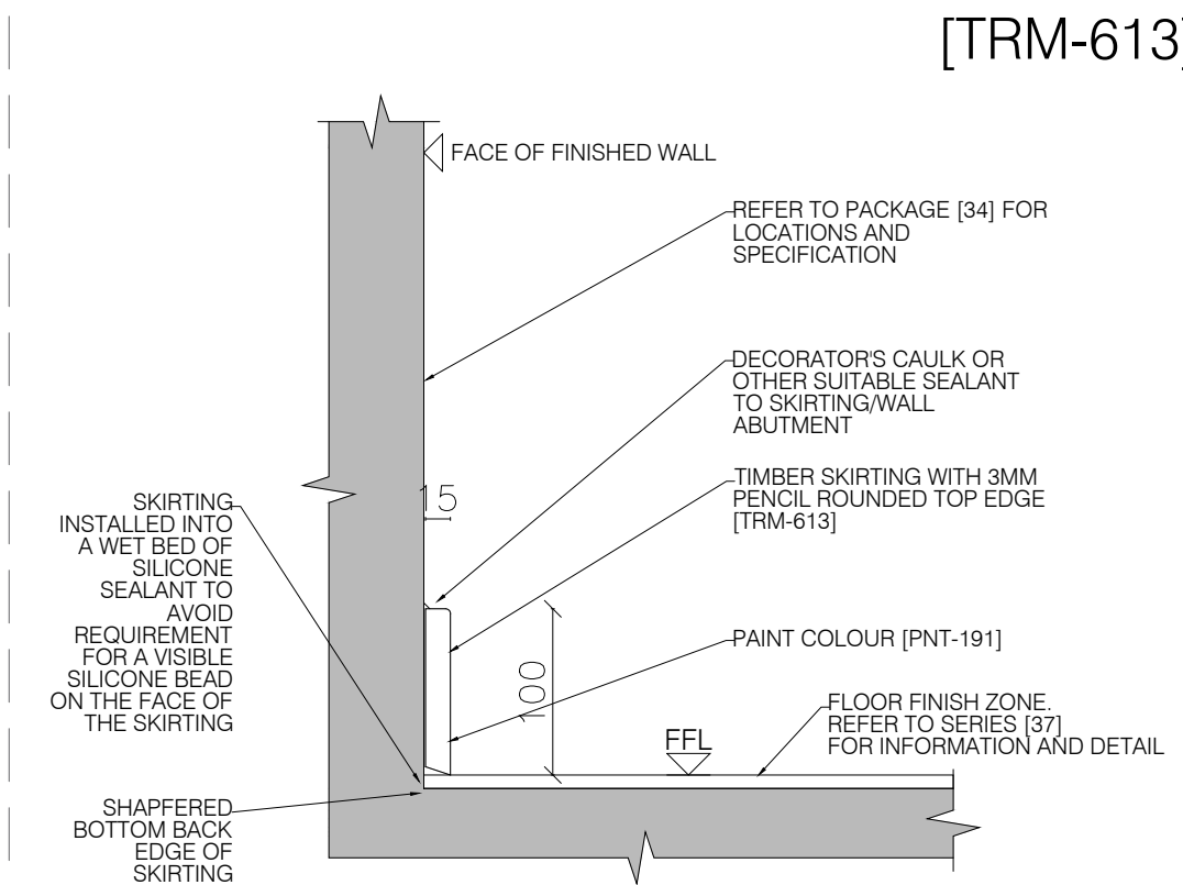
07 INTERNAL SKIRTING DETAIL - TYPE 3
