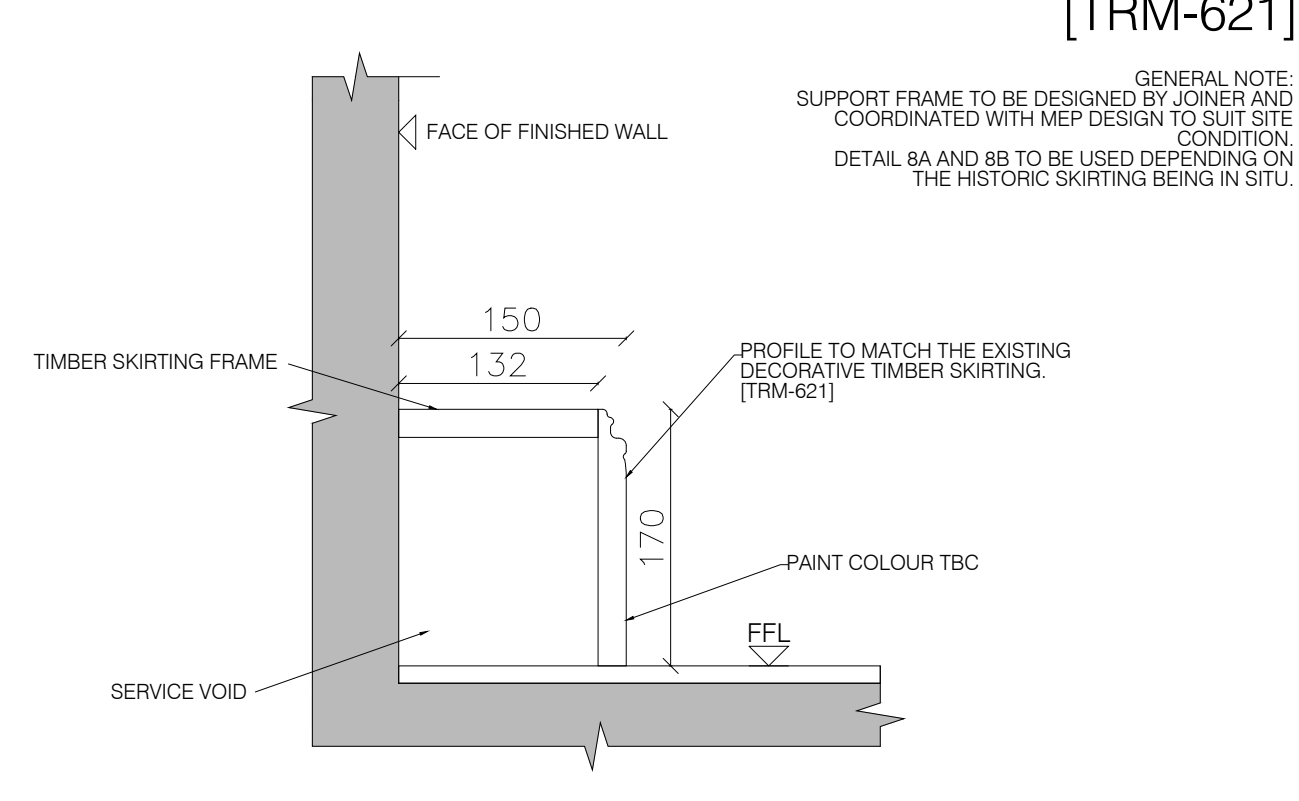
08A INTERNAL SKIRTING - TIMBER WITH SERVICES
