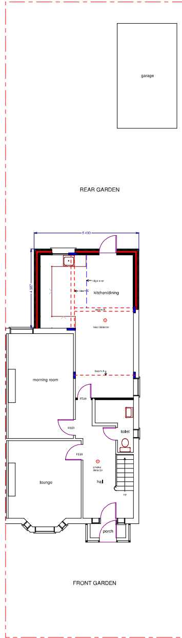
SITE PLAN AS EXISTING POST ERECTION OF SINGLE STOREY REAR EXTENSION.
