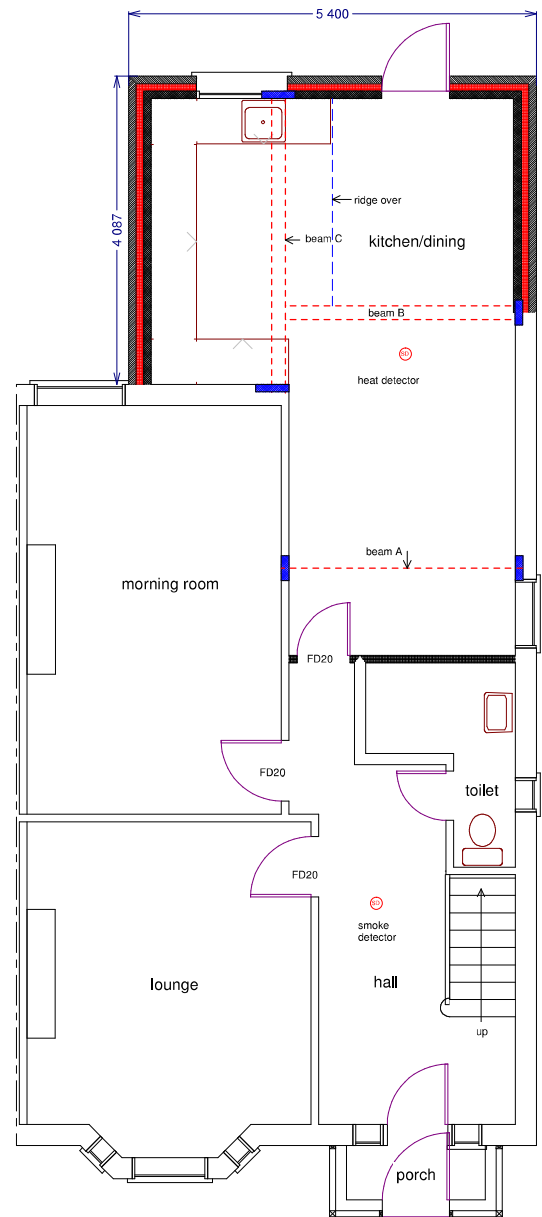
GROUND FLOOR PLAN AS EXISTING POST ERECTION OF SINGLE STOREY REAR EXTENSION.
