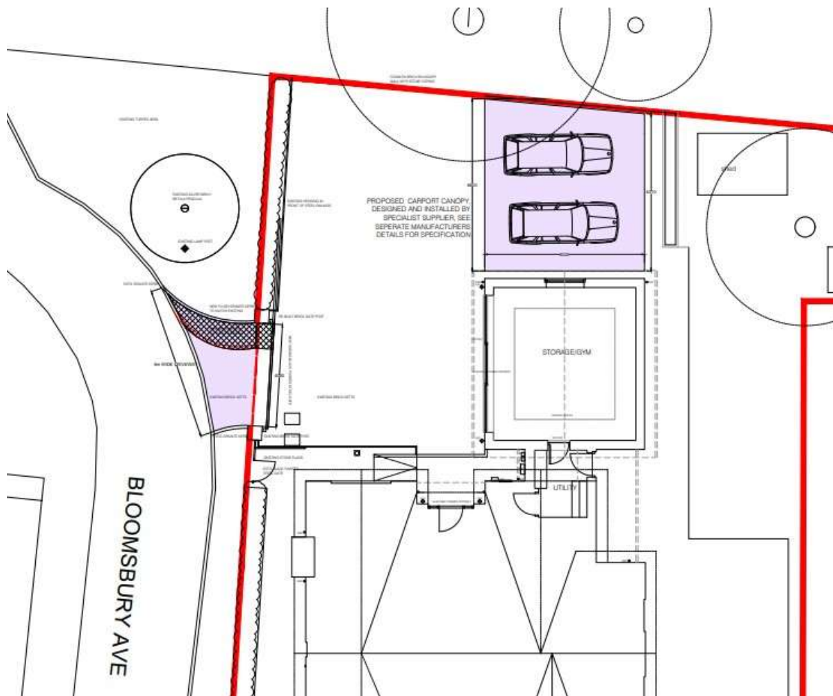
PROPOSED SITE PLAN INDICATING POSITION OF CAR PORT
