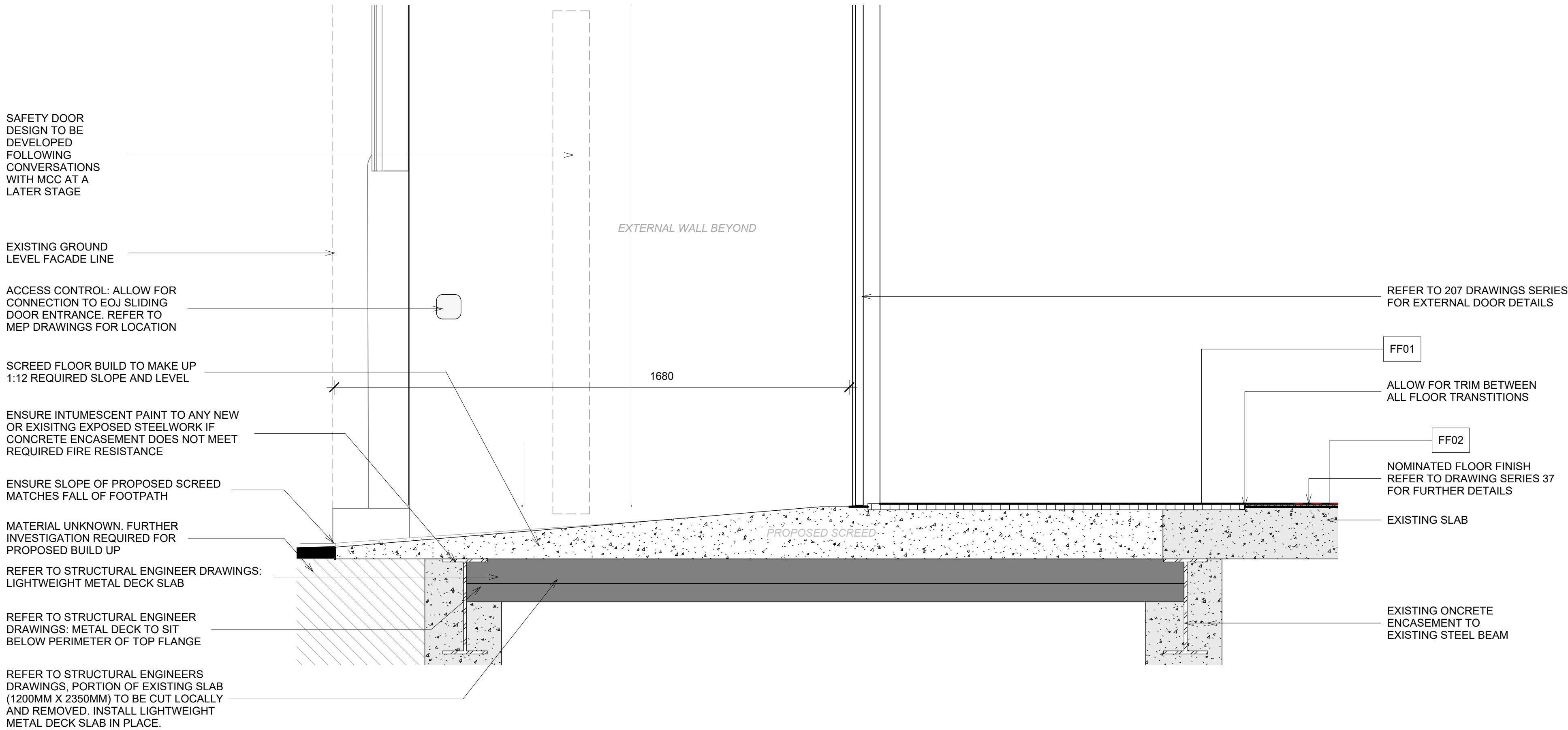
EOJ ENTRANCE SECTION A 1 : 10
