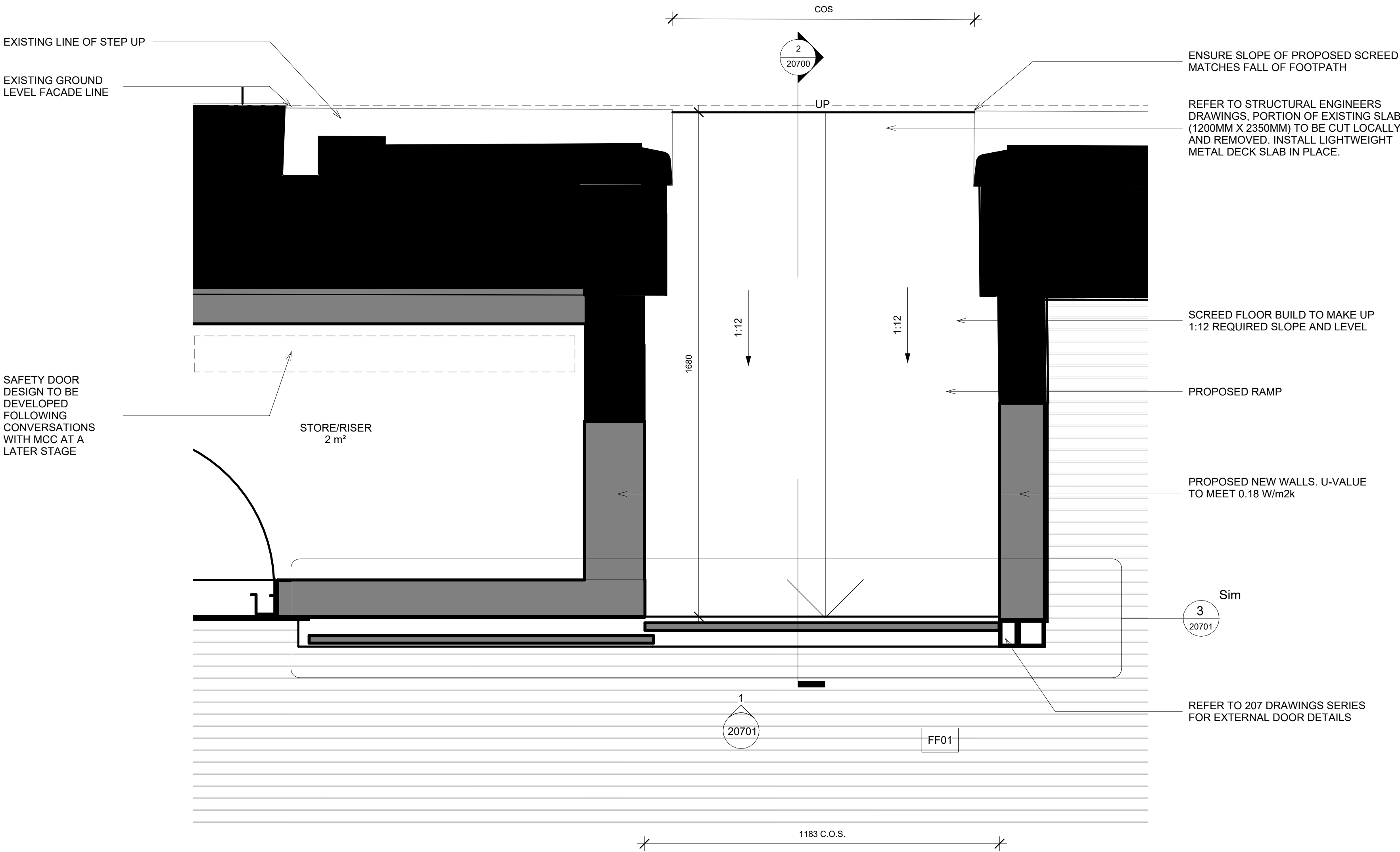
PROPOSED EOJ ENTRANCE PLAN LEVEL 00 1 : 10
