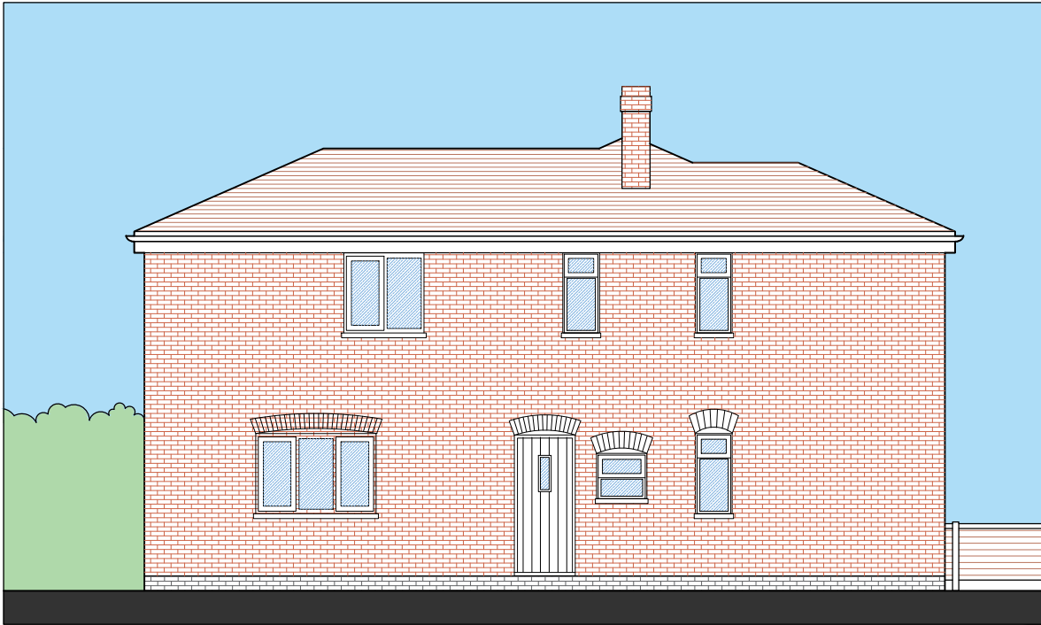
North Elevation
