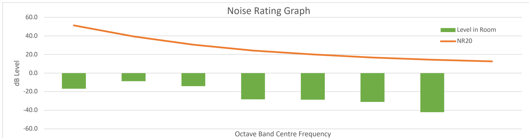
Figure 2: Predicted NR curve against NR20
