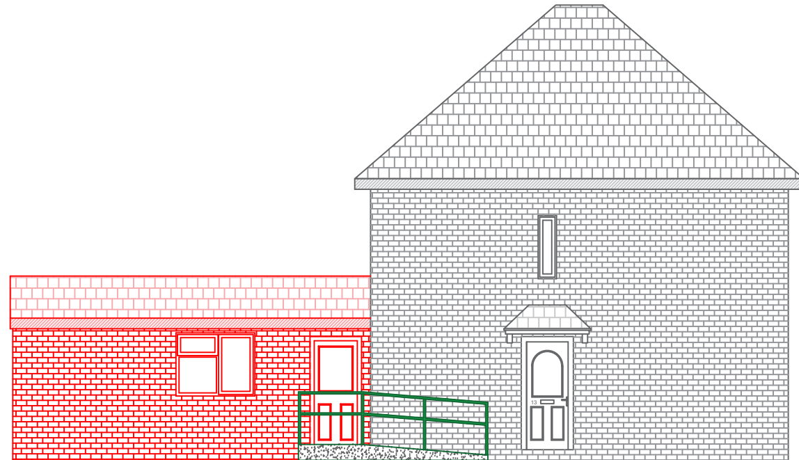
Proposed L/H/S elevation
