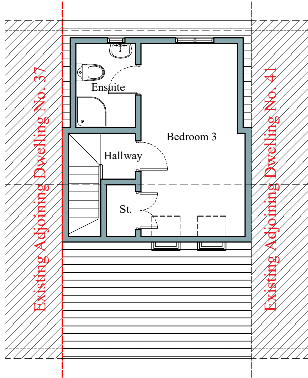
Proposed Loft Plan 1:100
