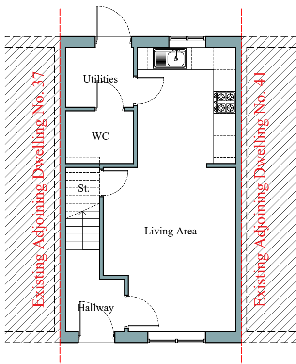
Proposed G/F Plan 1:100
