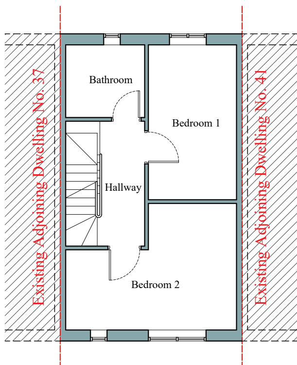
Proposed 1/F Plan 1:100
