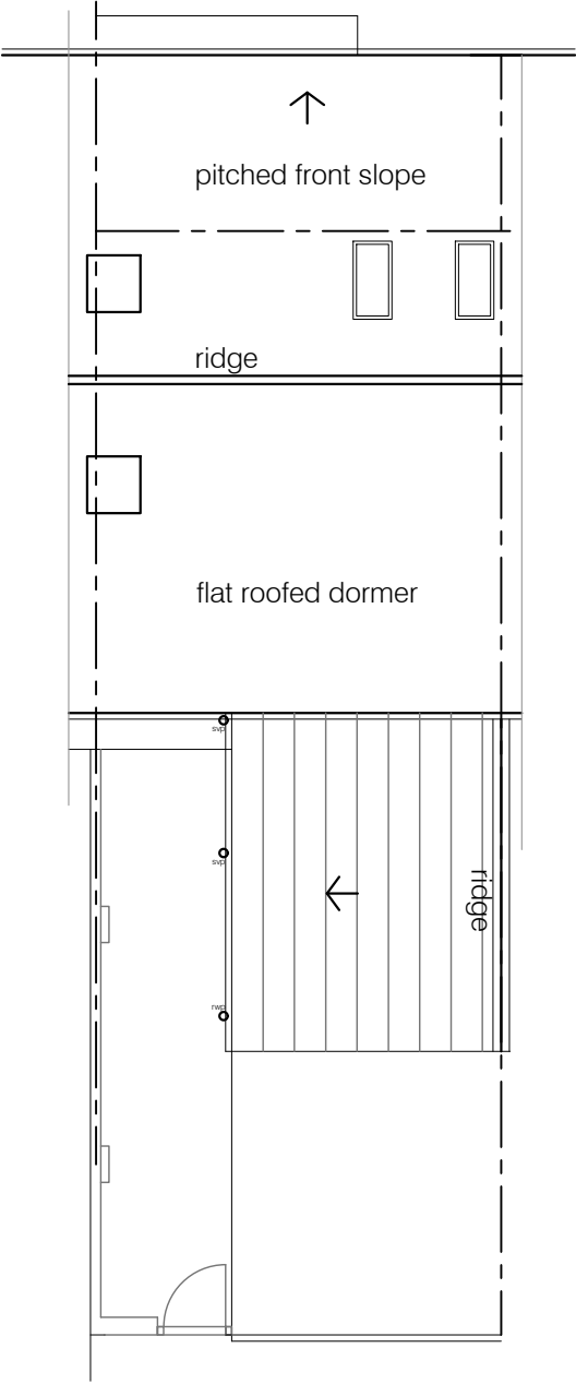
ROOF PLAN
