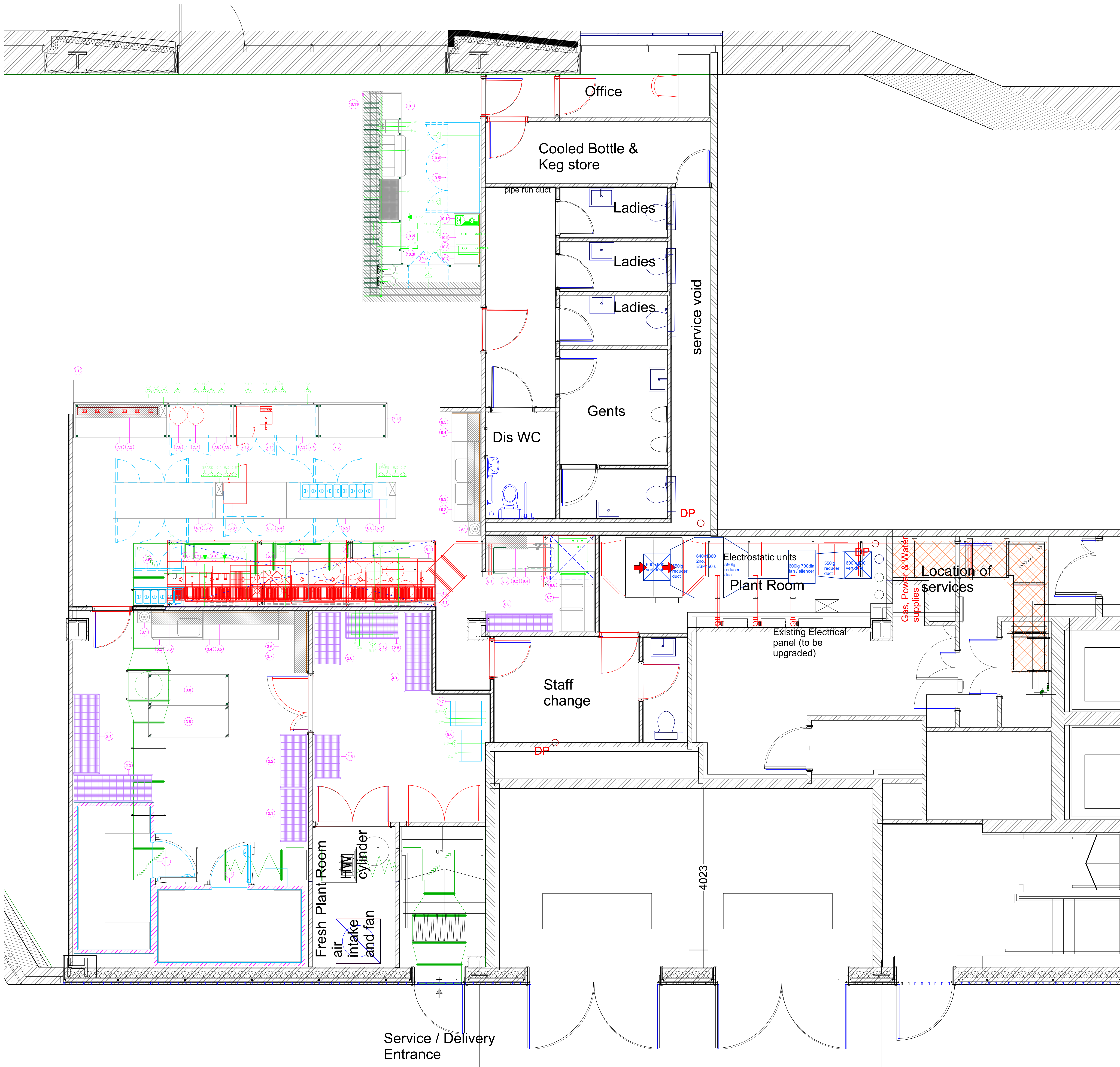
1 KITCHEN LAYOUT PLAN 1 : 30
