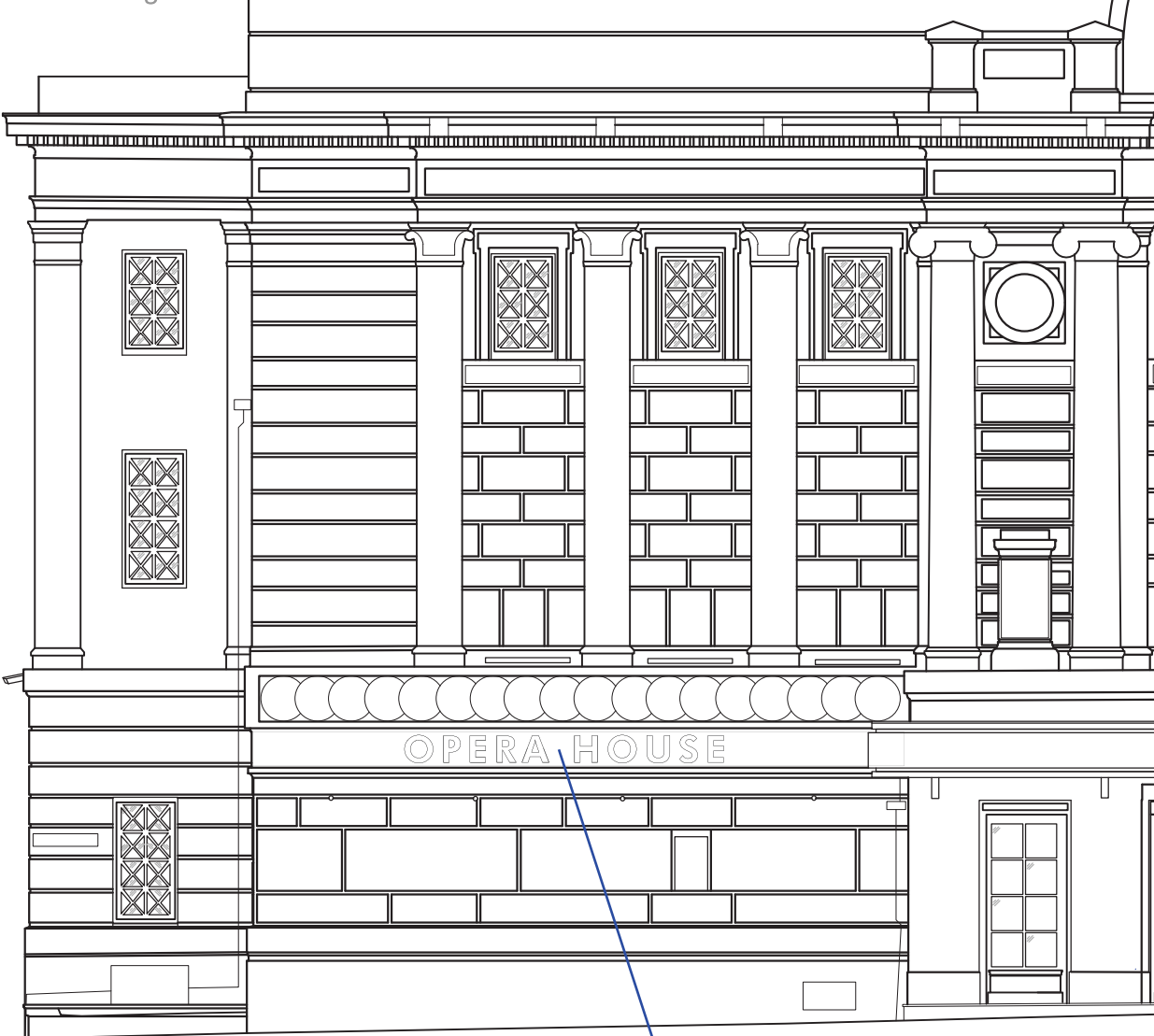
PROPOSED QUAY STREET ELEVATION 1:100
