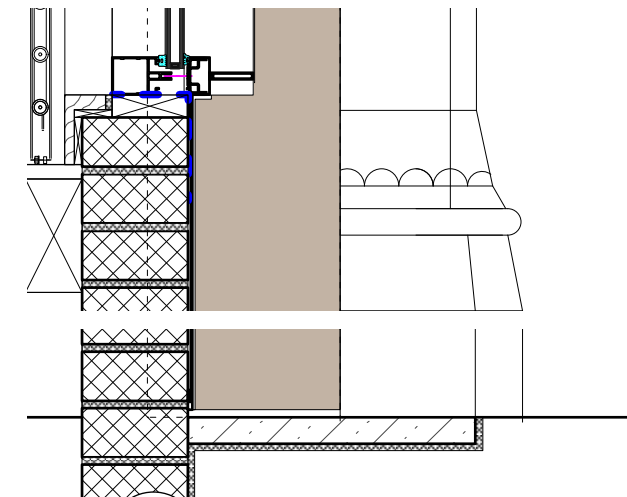
5 Proposed Shop Front Detail C Scale: 1:10
