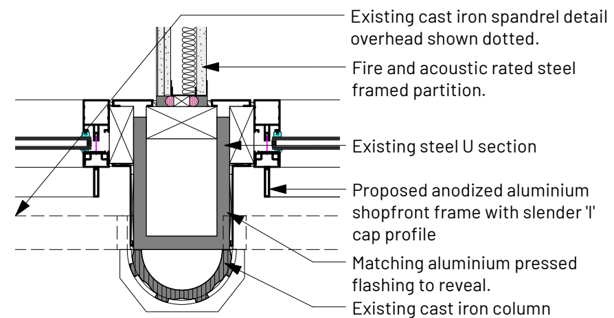
6 Proposed Shop Detail A Scale: 1:10
