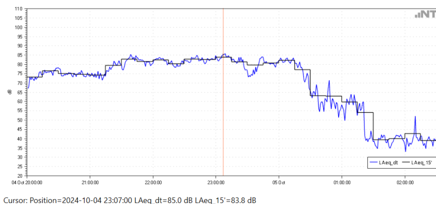
Figure 3 Internal measured noise levels
