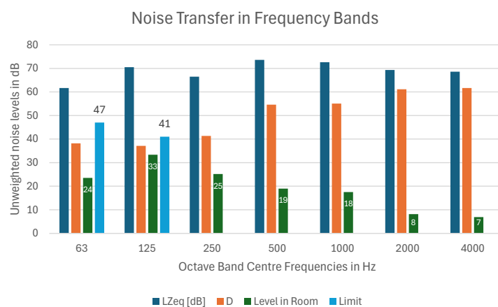
Figure 4 Noise Transfer in frequency bands
