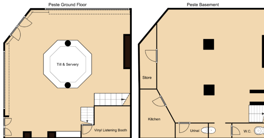
Figure 3 As Built floor plans
