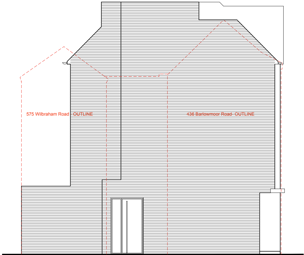
SIDE ELEVATION (TO COURTYARD)
