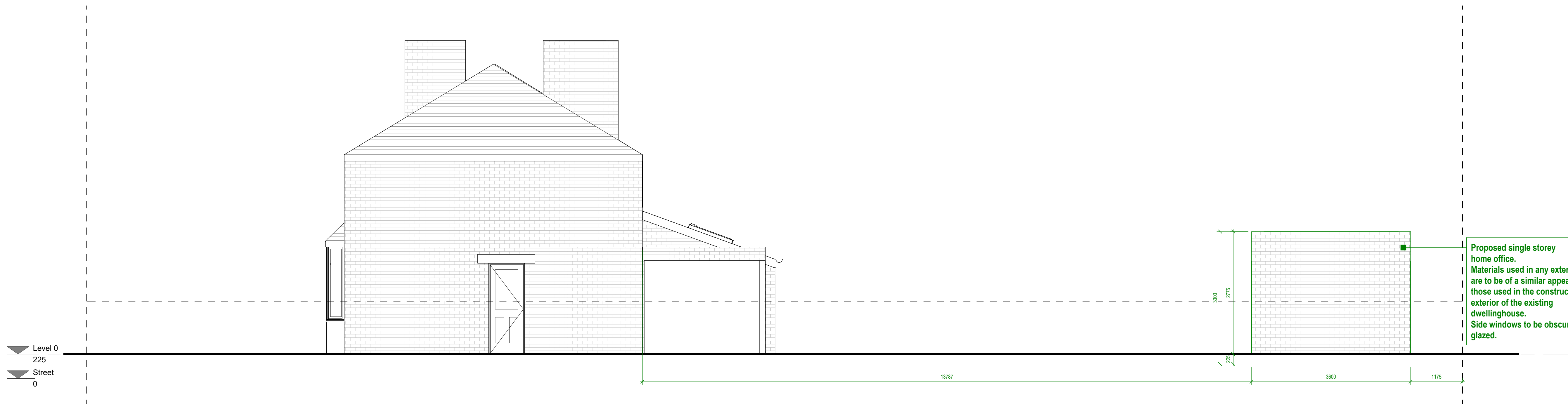
2 Proposed Side 1 Elevation 1 : 50
