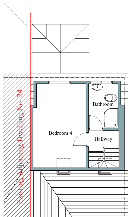
Proposed Loft Plan 1:100
