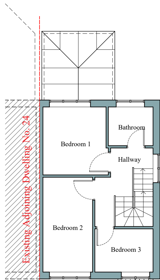
Proposed 1/F Plan 1:100
