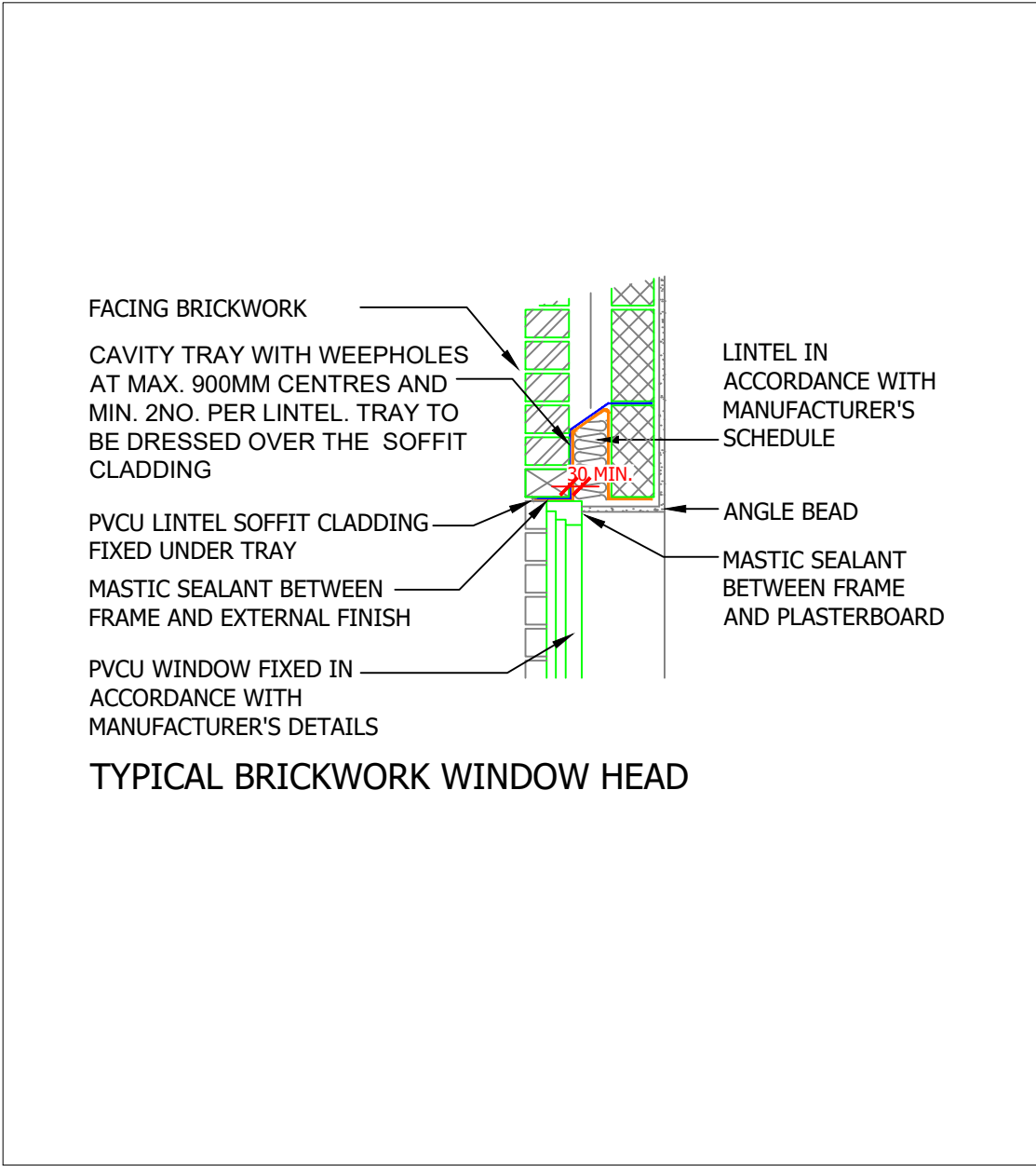
11- Brickwork and Window Head
