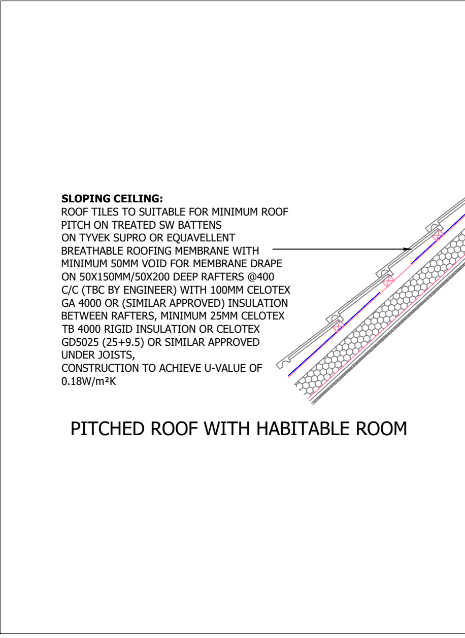
10- Pitched Roof Detail
