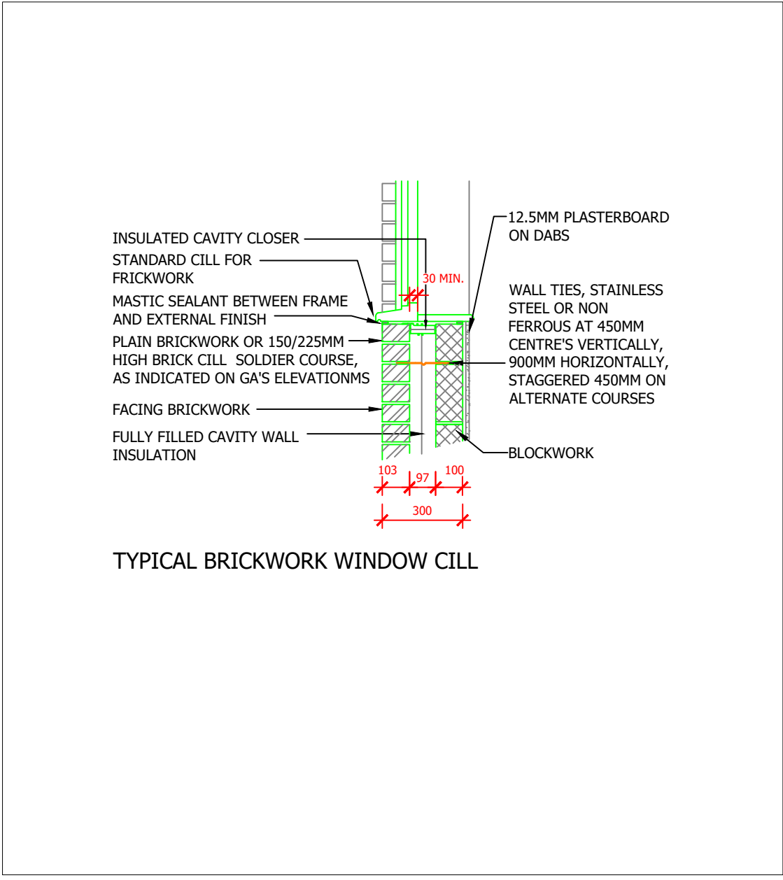
12- Brickwork Window Cill
