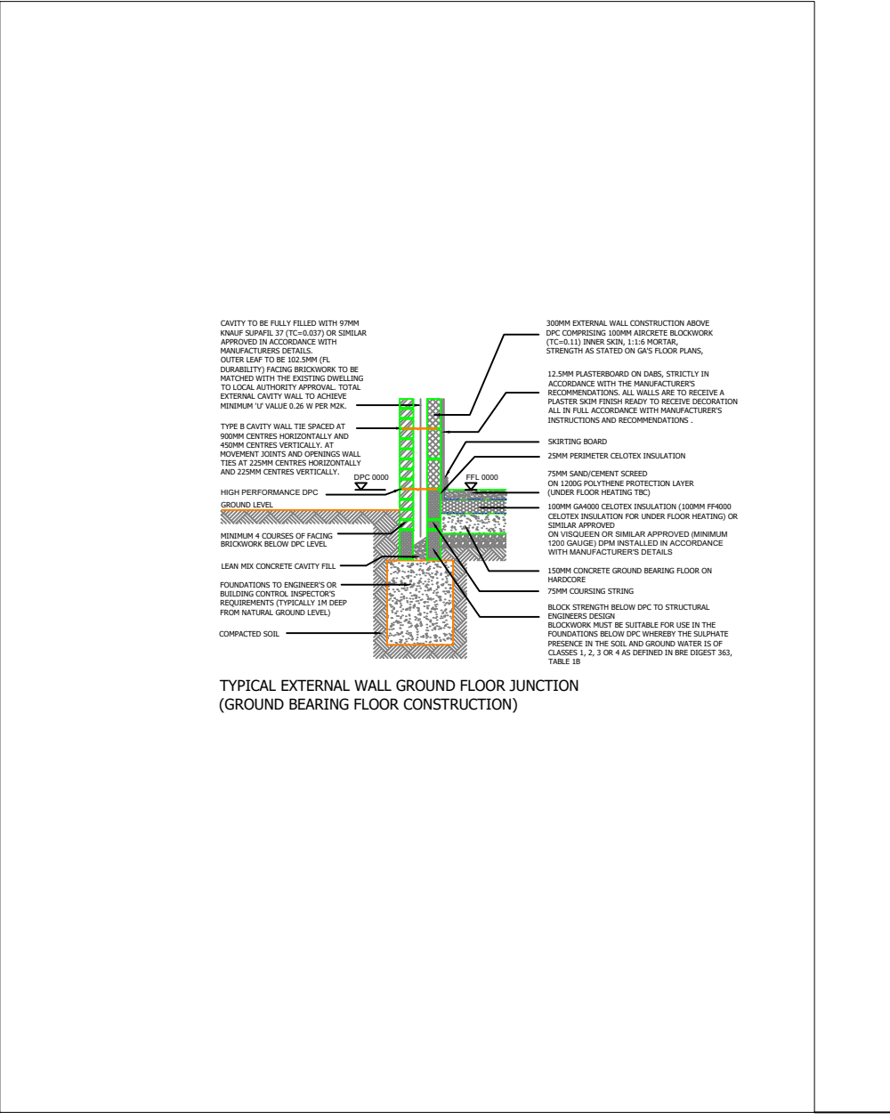
8- Foundation Detail
