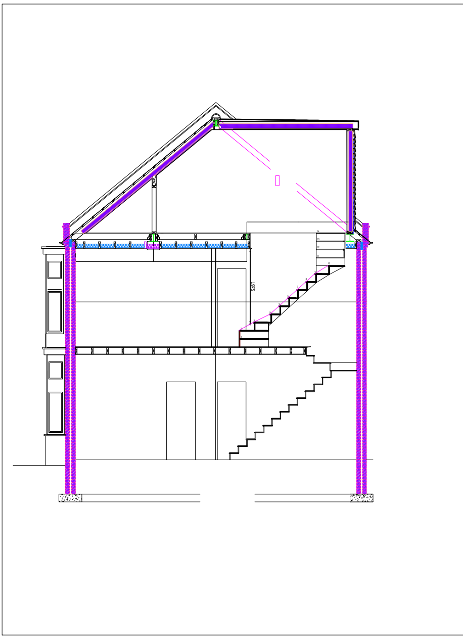
1- X- Sec.for information only (not scale)
