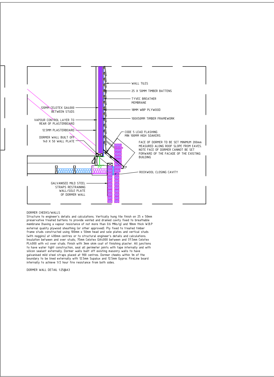
5- Dormer Wall Detail for information only (not scale)
