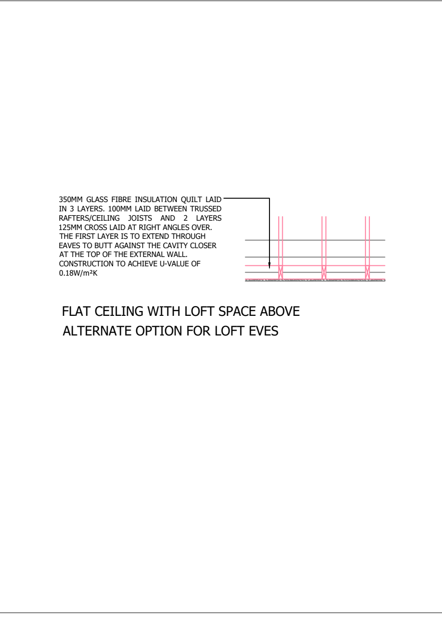
9- Flat Ceiling with Loft
