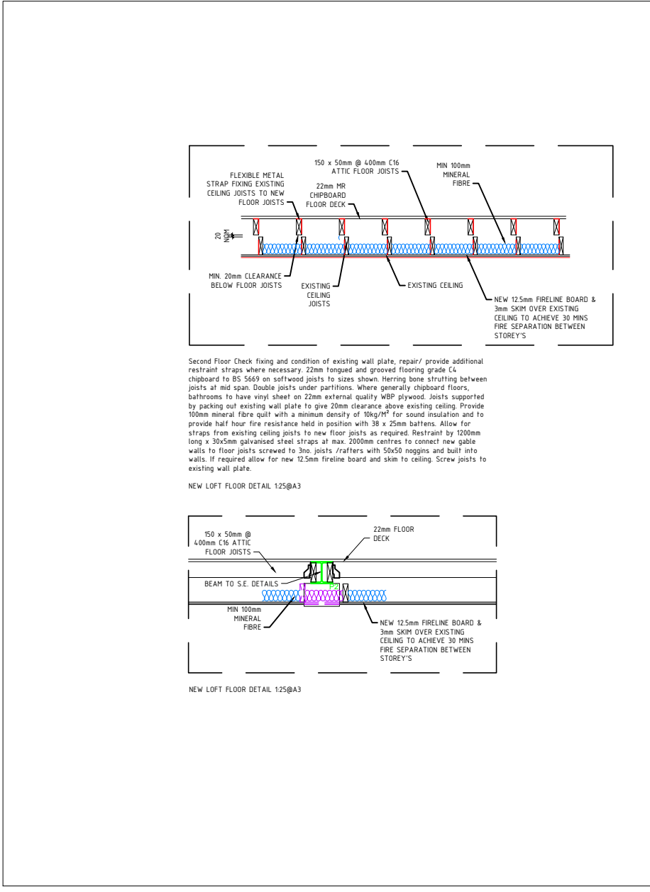
6- New Floor Details
