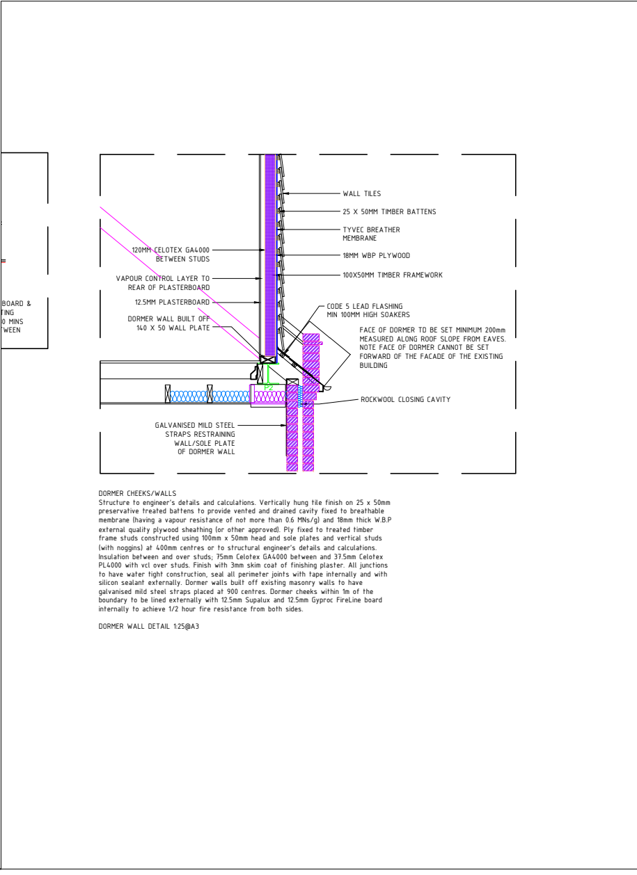
7- Dormer Wall Detail
