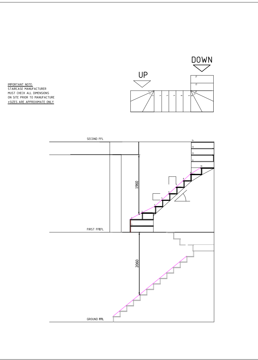
4- Stair Case Details
