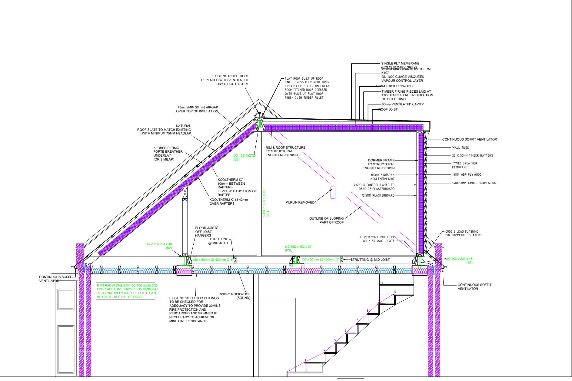
13- X- Sec B. for information only (not scale)
