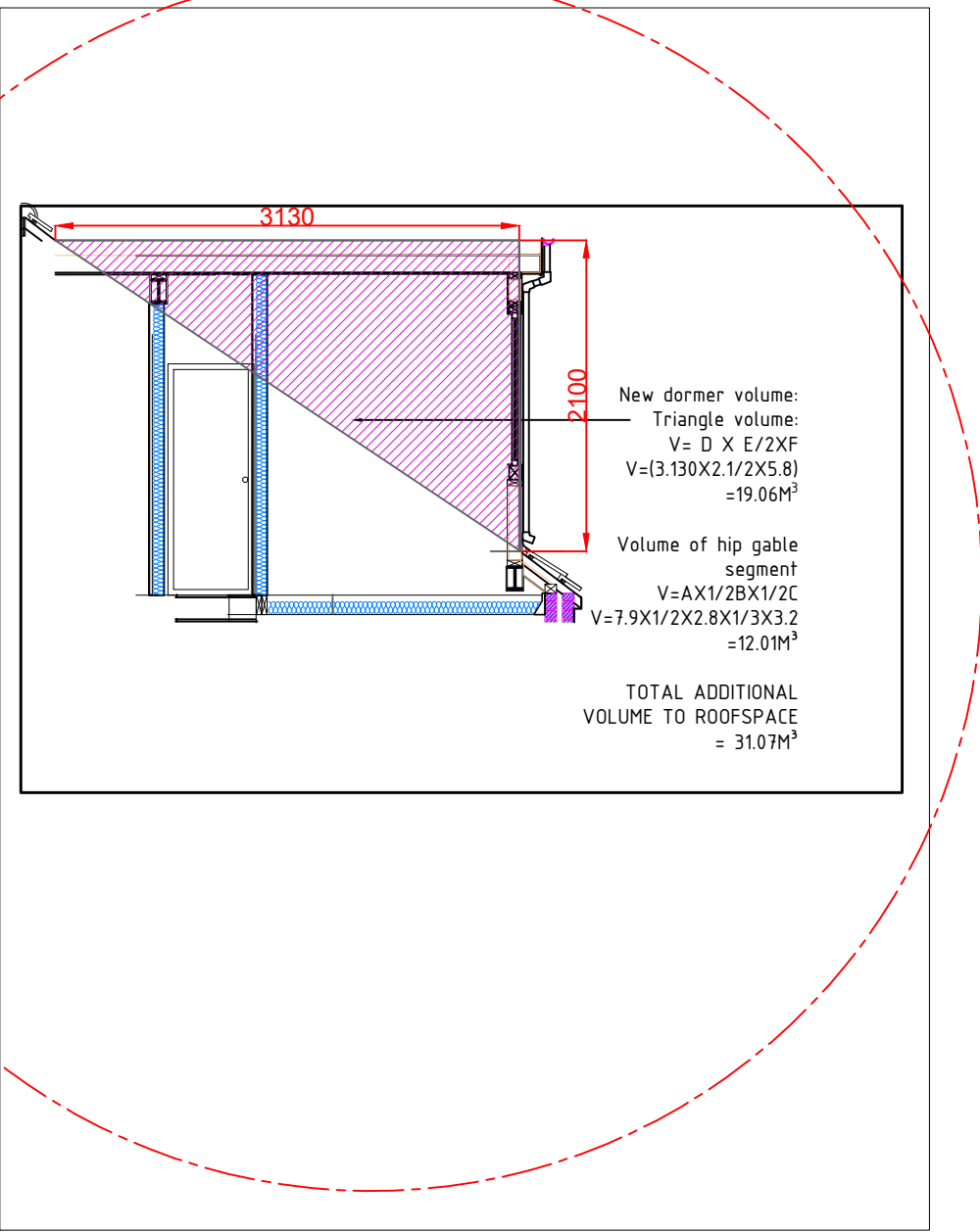
3- Volume Calculation
