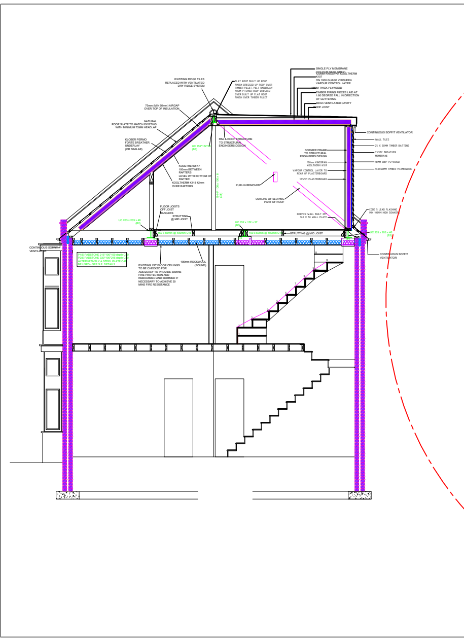
2- X- Sec and Details for information only (not scale)
