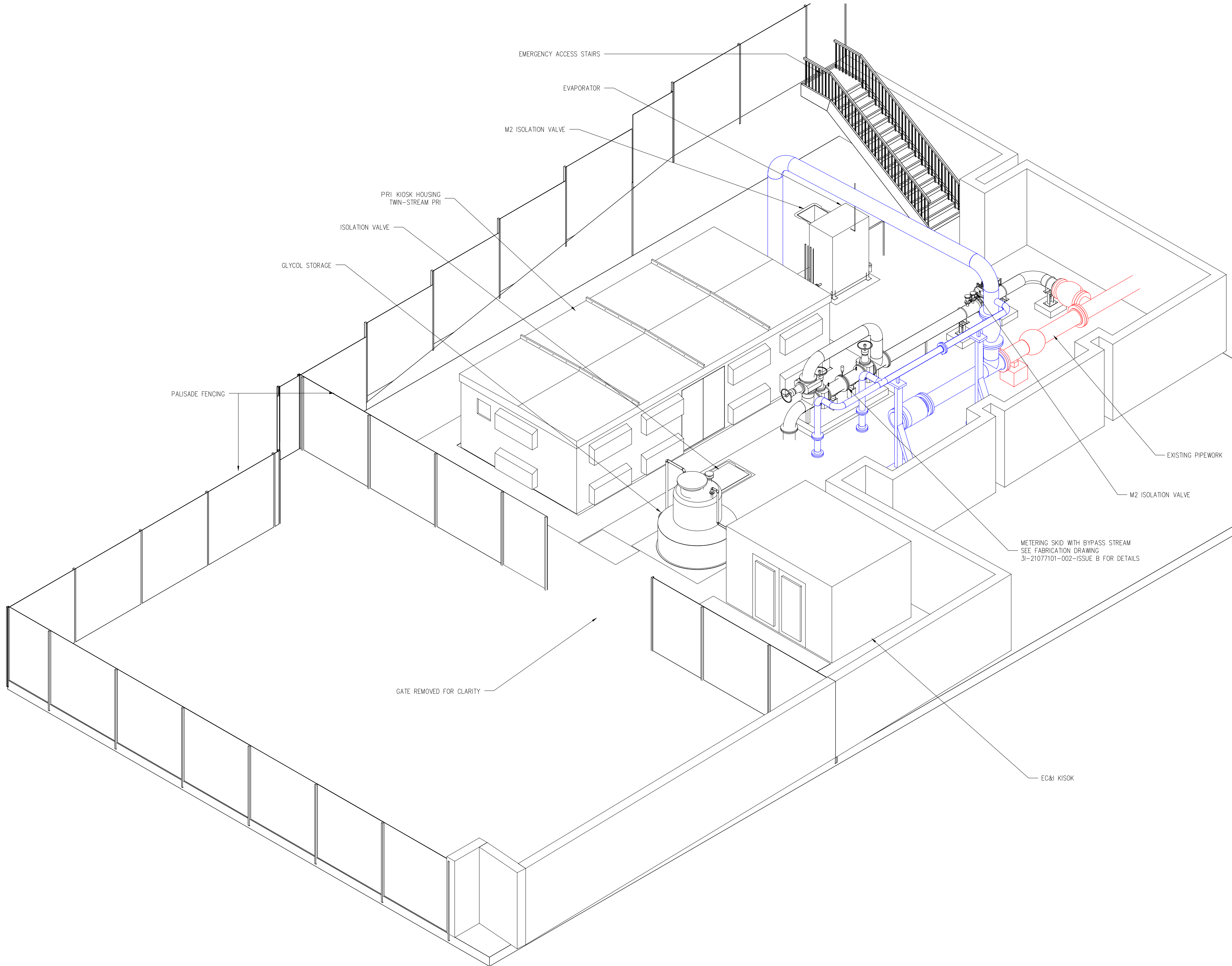
ISOMETRIC VIEW (SCALE 1:50)
