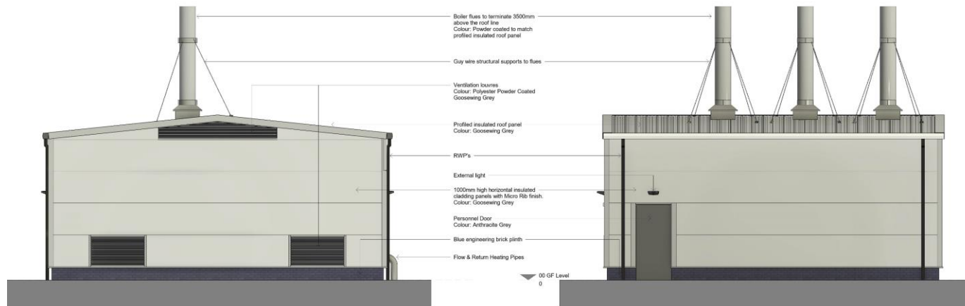
Proposed South East Facing Elevation
