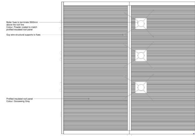
Roof Plan
