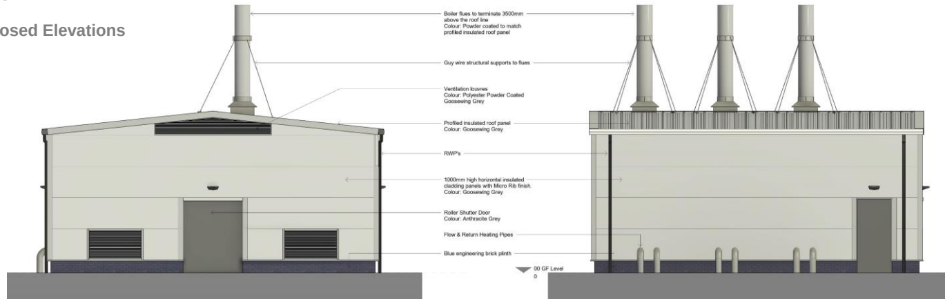
Proposed North West Facing Elevation
