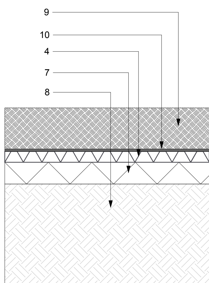
8 Top Soil on Solid Ground Scale: 1:10
