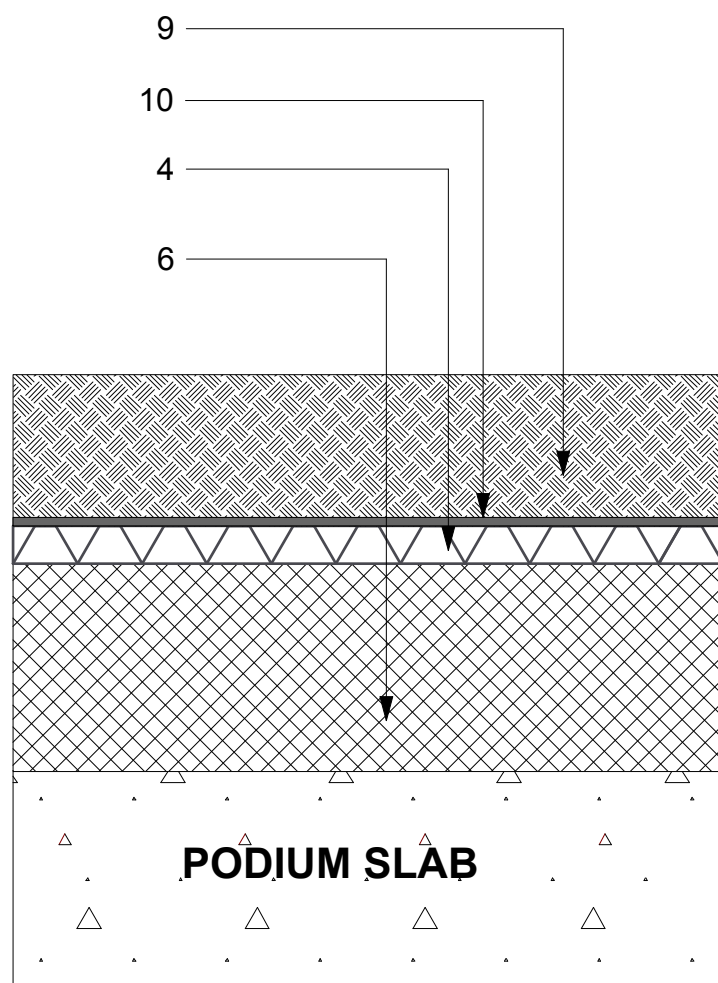
7 Top Soil on Insulated Areas Scale: 1:10
