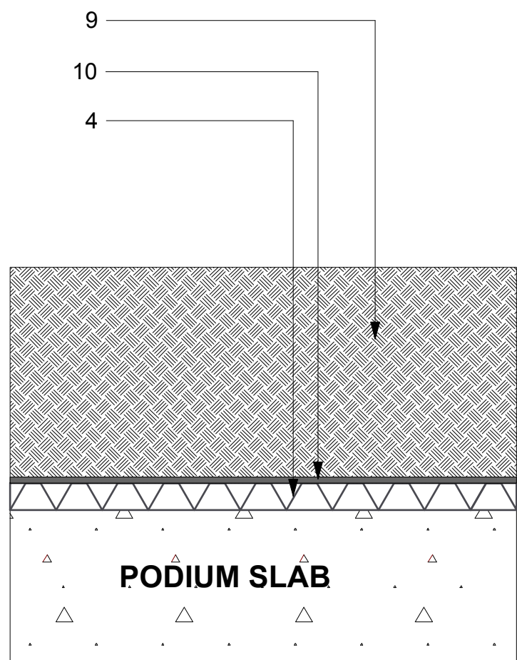
6 Top Soil To Non Insulated Areas Scale: 1:10
