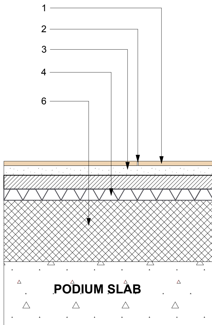
3 Build Up on Insulation Scale: 1:10
