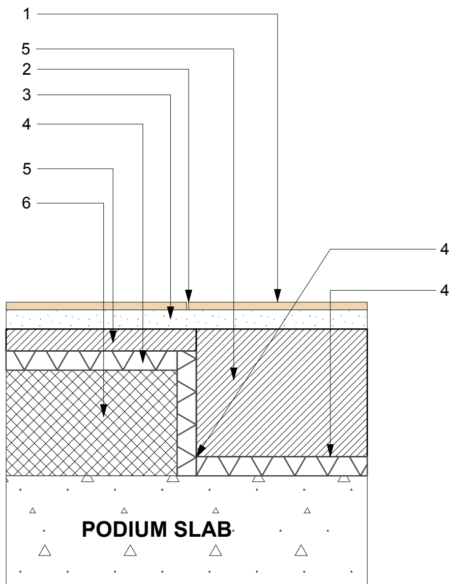
5 Void Forma & Insulation Junction Scale: 1:10
