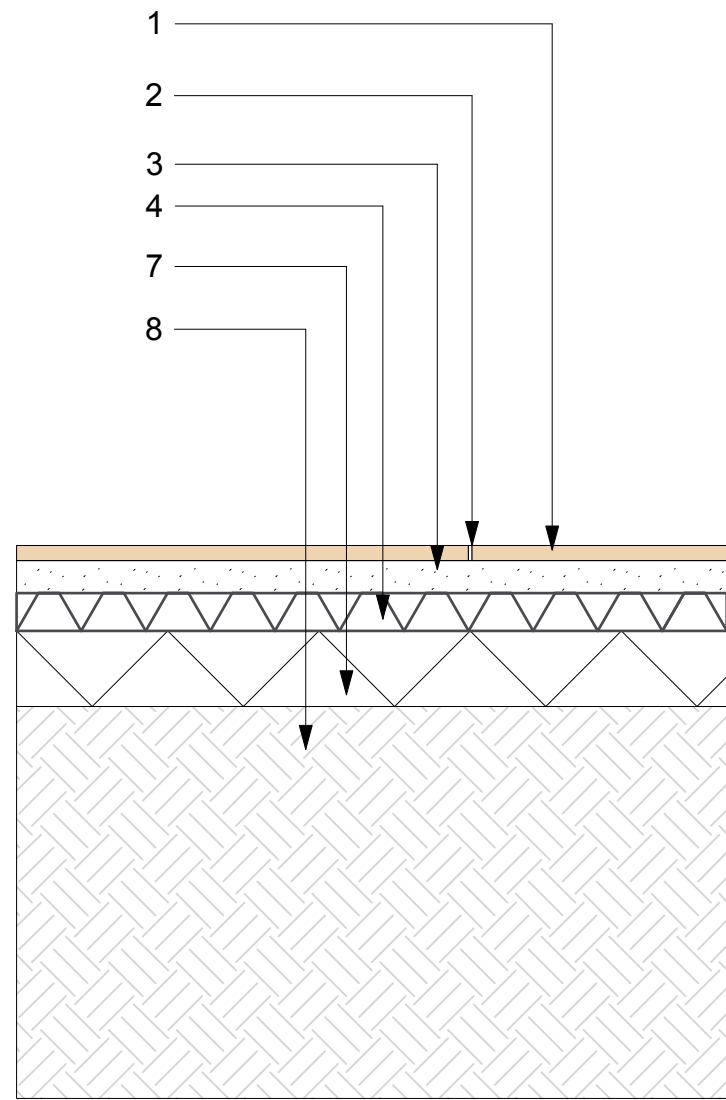
4 Build Up on Soild Ground Scale: 1:10
