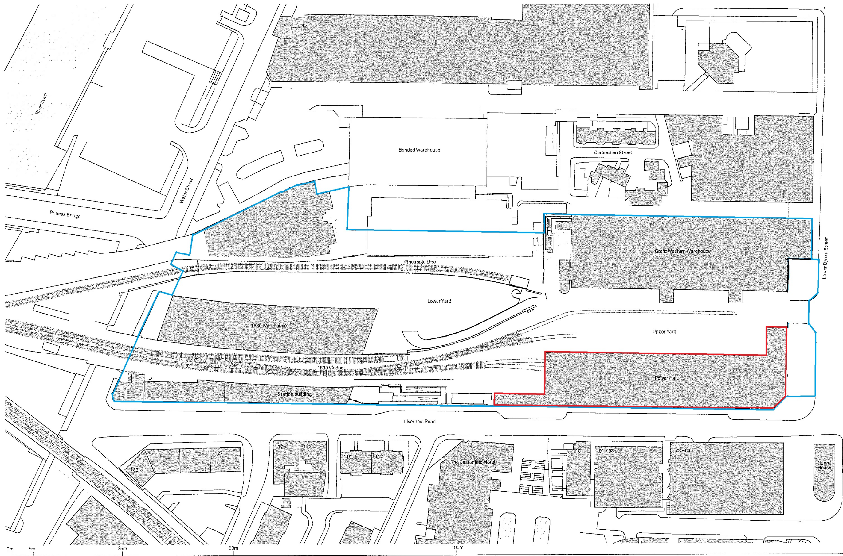
Museum of Science and Industry, Site Plan 1:500
