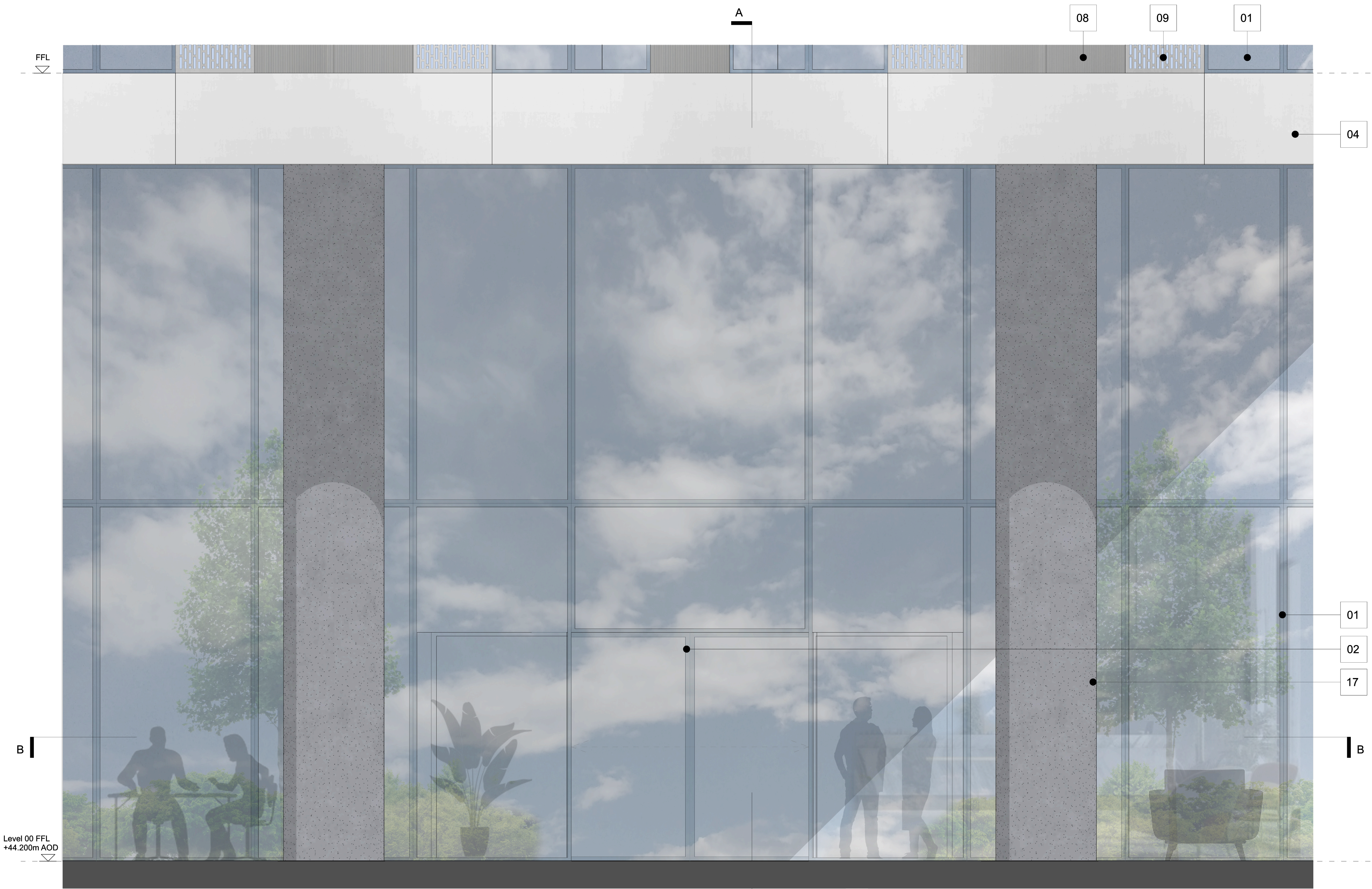
Detail Elevation 1:25
