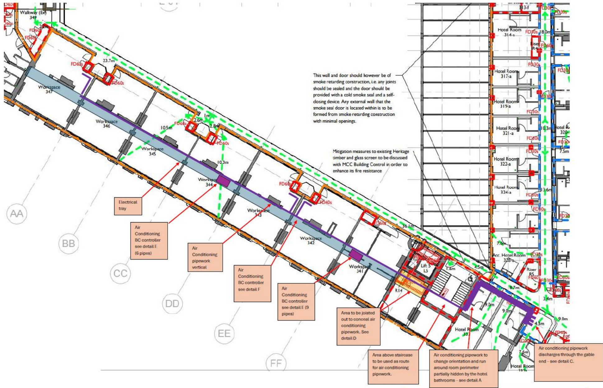
Section of Third Floor Plan – Air Conditioning Route Fairfield Street
